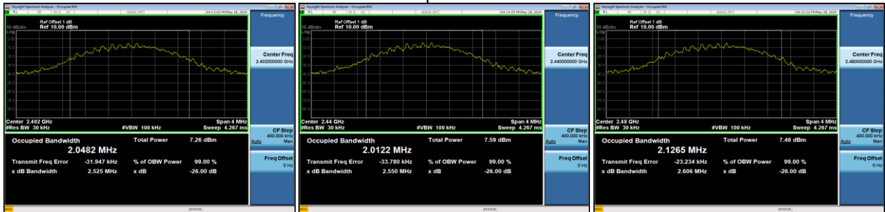
99 % Occupied Bandwidth
