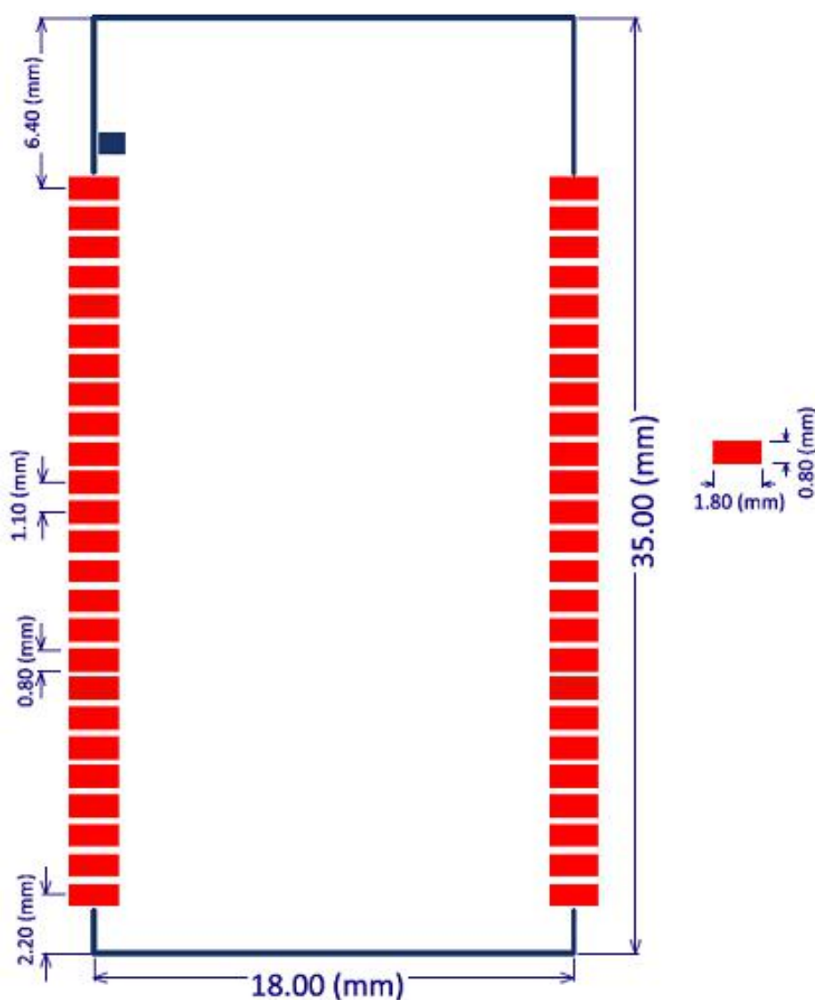
Figure 4. Footprint dimensions
