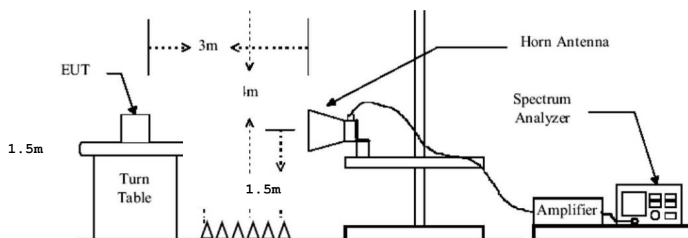
Test setup for 1-25GHz
