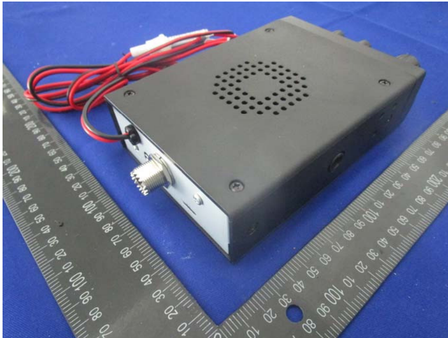
EUT –CB91 L Side View
