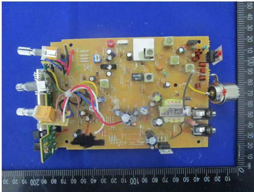
EUT –CB91 L Main Board Top View
