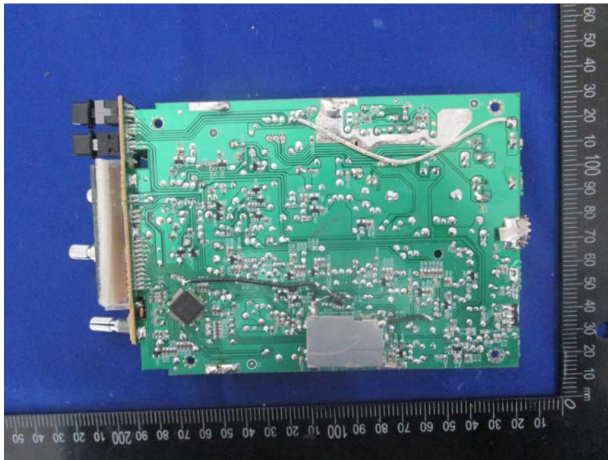
EUT – CB91 Main Board Bottom View
