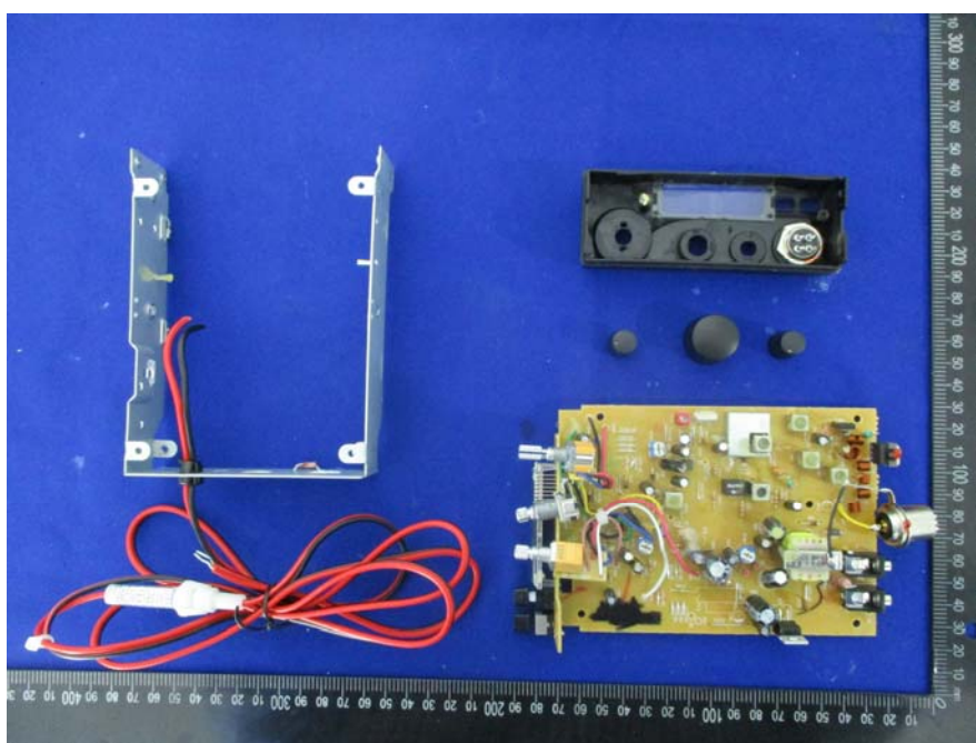
EUT –CB91 L Uncover-2 View
