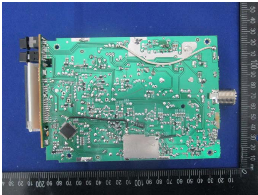
EUT –CB91 L Main Board Bottom View
