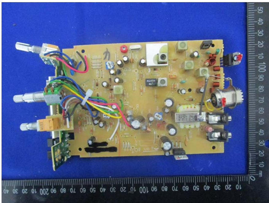
EUT –CB91 Main Board Top View
