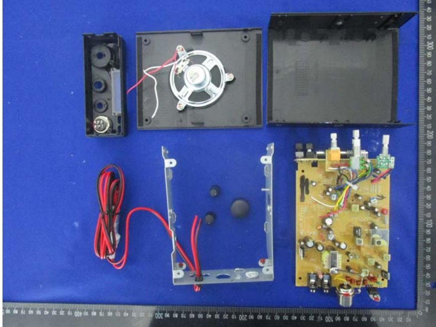
EUT – CB91 Uncover View
