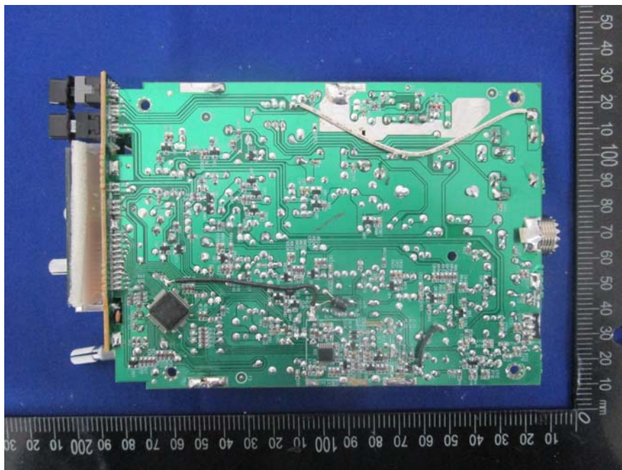
EUT –CB91 Main Board Botton Uncover View
