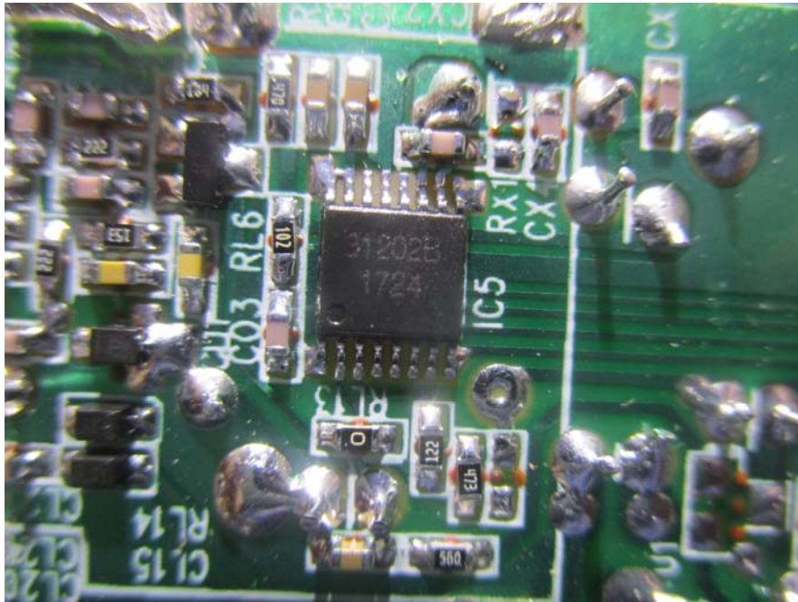
EUT –CB91 L Chip View
