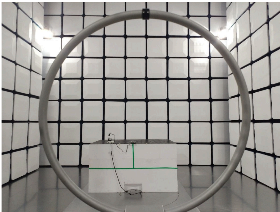
Below 30MHz-BT/BLE
