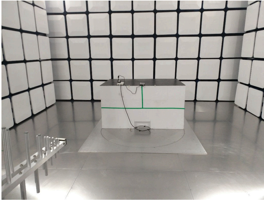
Blow 1GHz-BT/BLE
