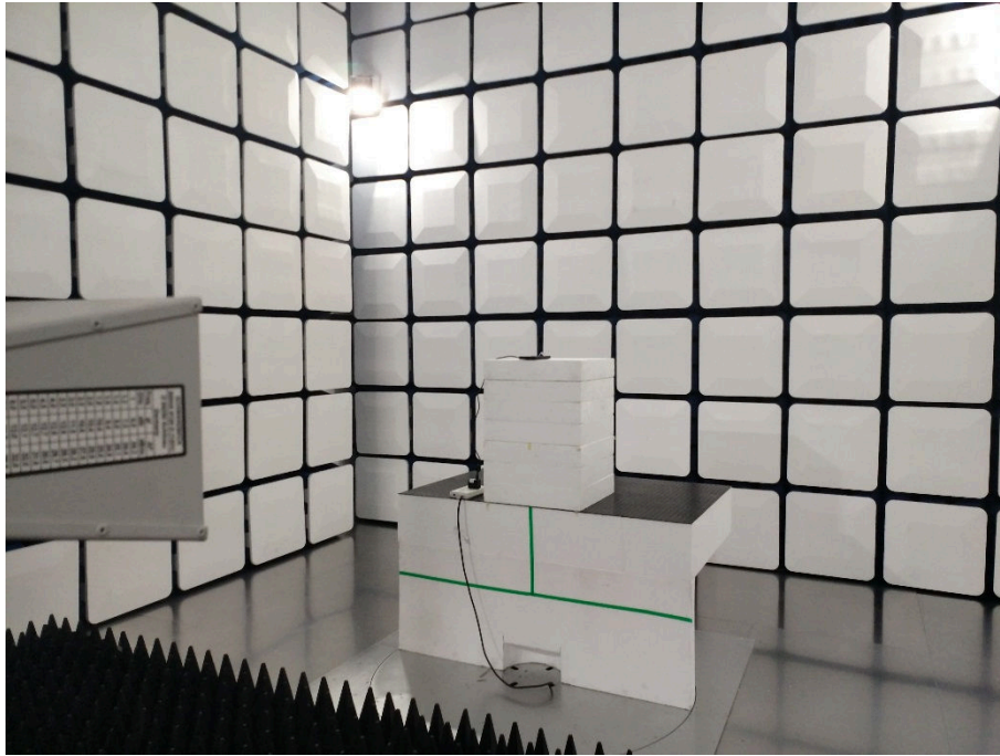
Above 1GHz-BT/BLE
