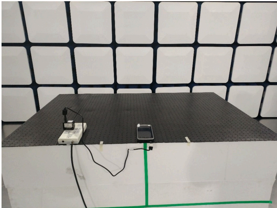
Close-up-BT/BLE
