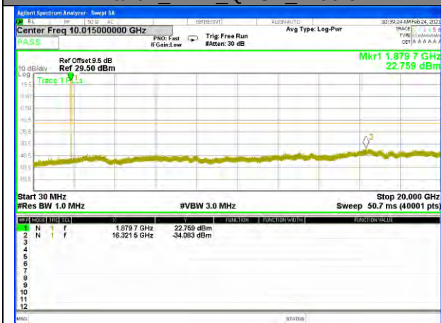
Band2_1.4M_QPSK_High
