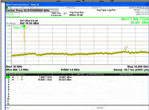
Band2_1.4M_QPSK_High
