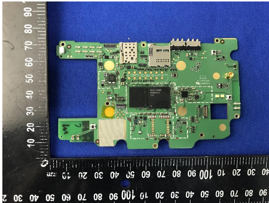
MAIN BOARD TOP VIEW WITHOUT RF MODULE
