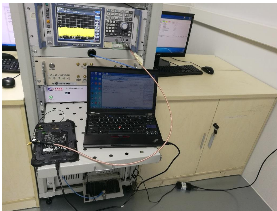
Conducted Test-BT4.0
