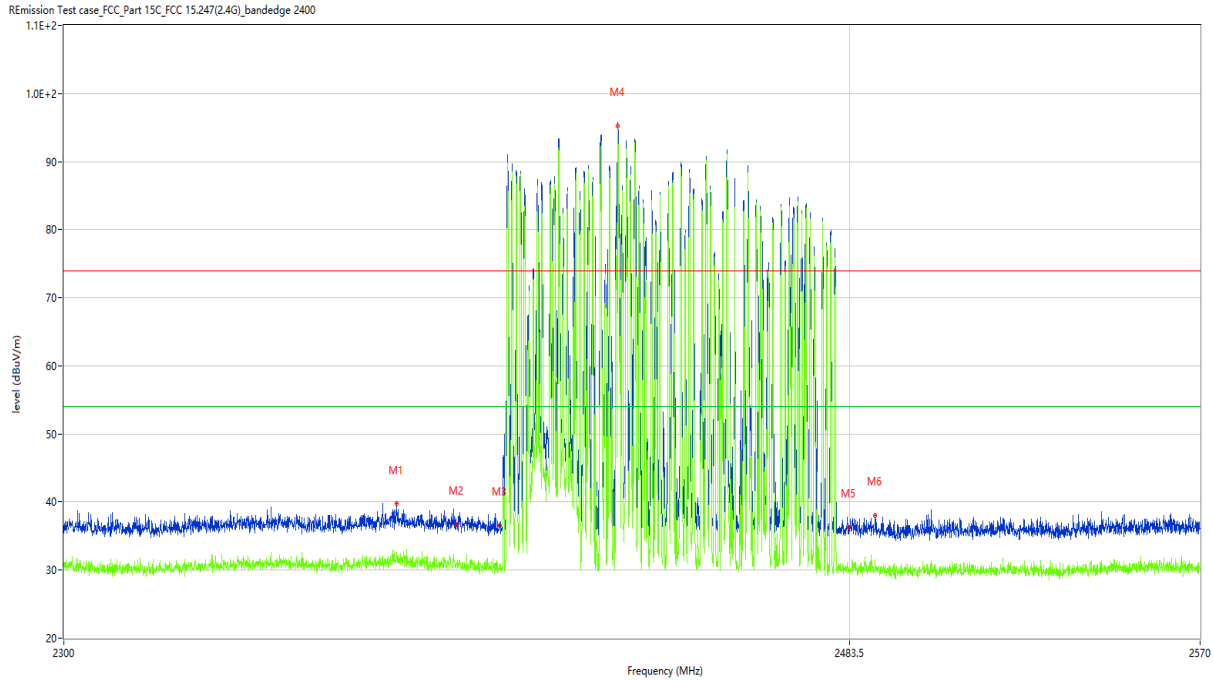
Figure 38: Band Edge (Restricted-band band-edge), Hopping Mode, 8-DPSK Horizontal
