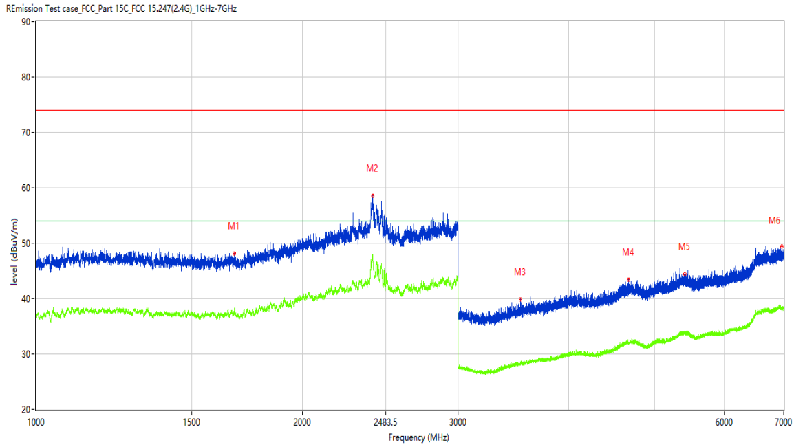
Figure 32: Spurious Emission, 1GHz – 10 th Harmonic, Hopping Mode, 8-DPSK 1GHz-7GHz, Horizontal
