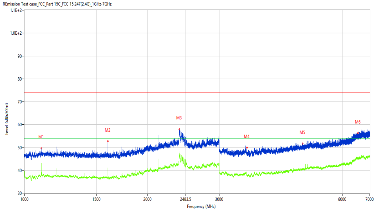
Figure 31: Spurious Emission, 1GHz – 10 th Harmonic, Hopping Mode, GFSK 1GHz-7GHz, Horizontal
