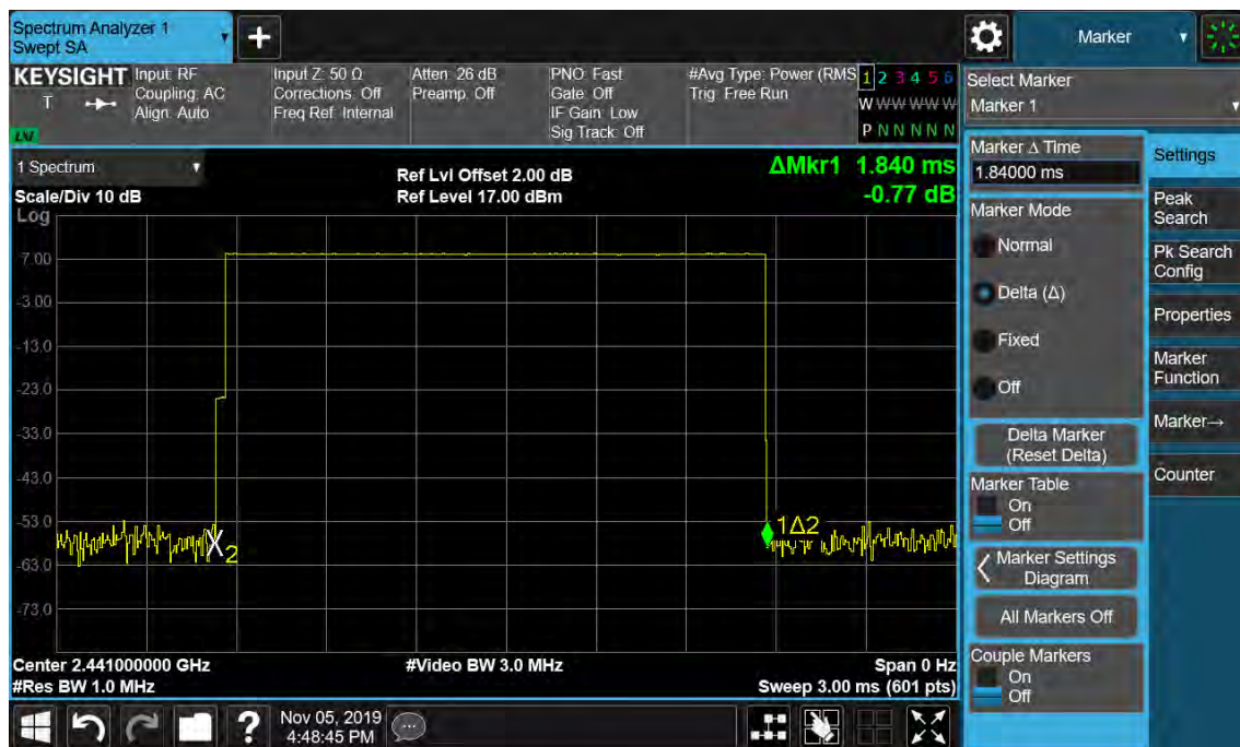
Figure 44: Time of Occupancy, 2441MHz, GFSK DH3
