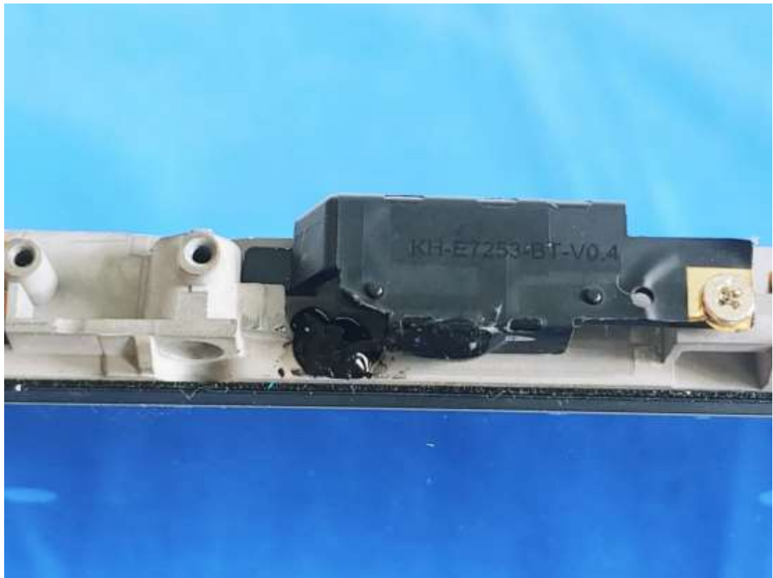
WIFI BT antenna 1
