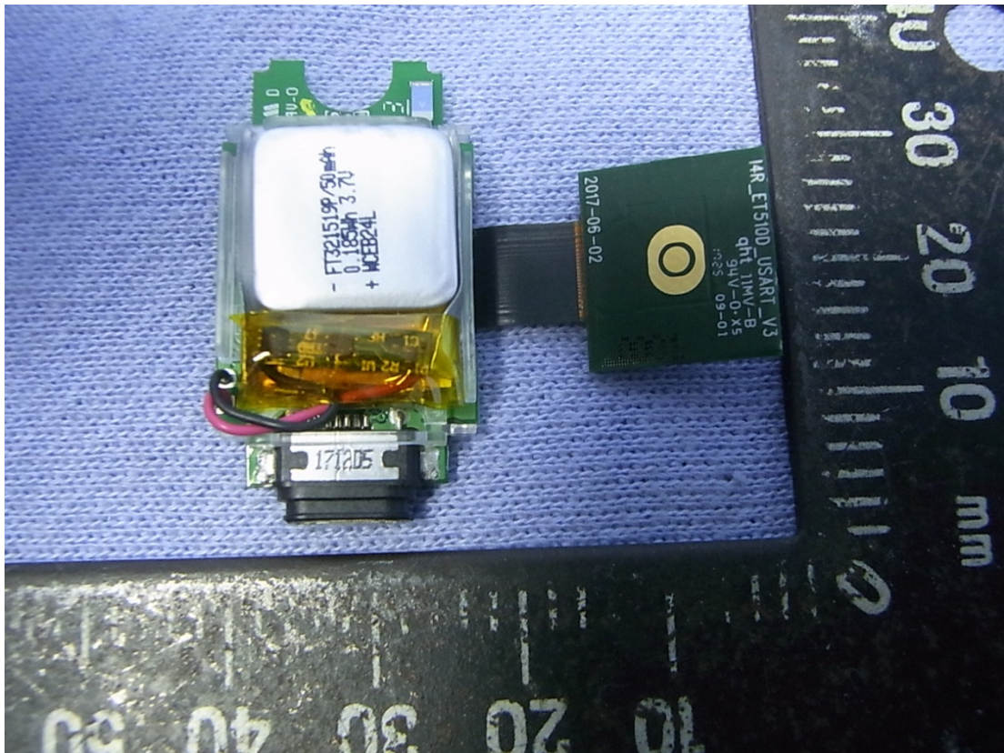
Figure 6 Internal View (Main Board/Front View, Touch Board/Back View)
