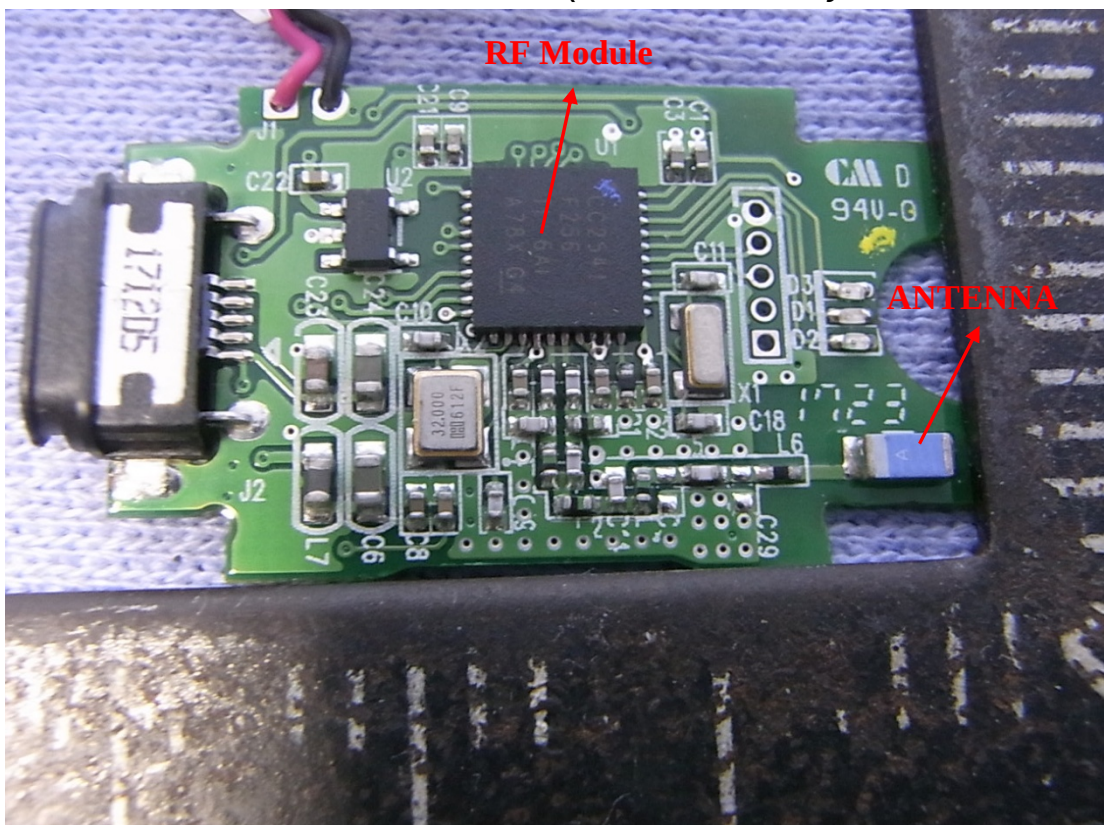
Figure 7 Internal View (Removed Battery, Main Board/Front View)
