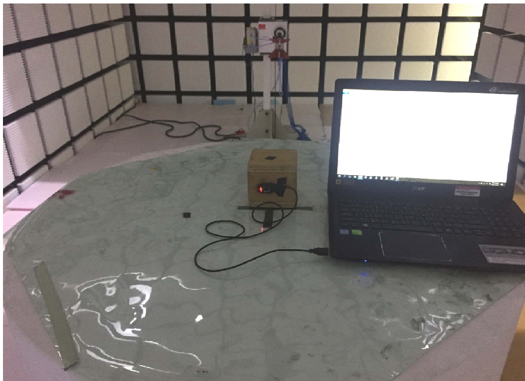
EUT on Side
