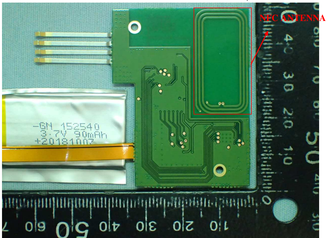
Figure 12 Internal View (Main Board/Front View)
