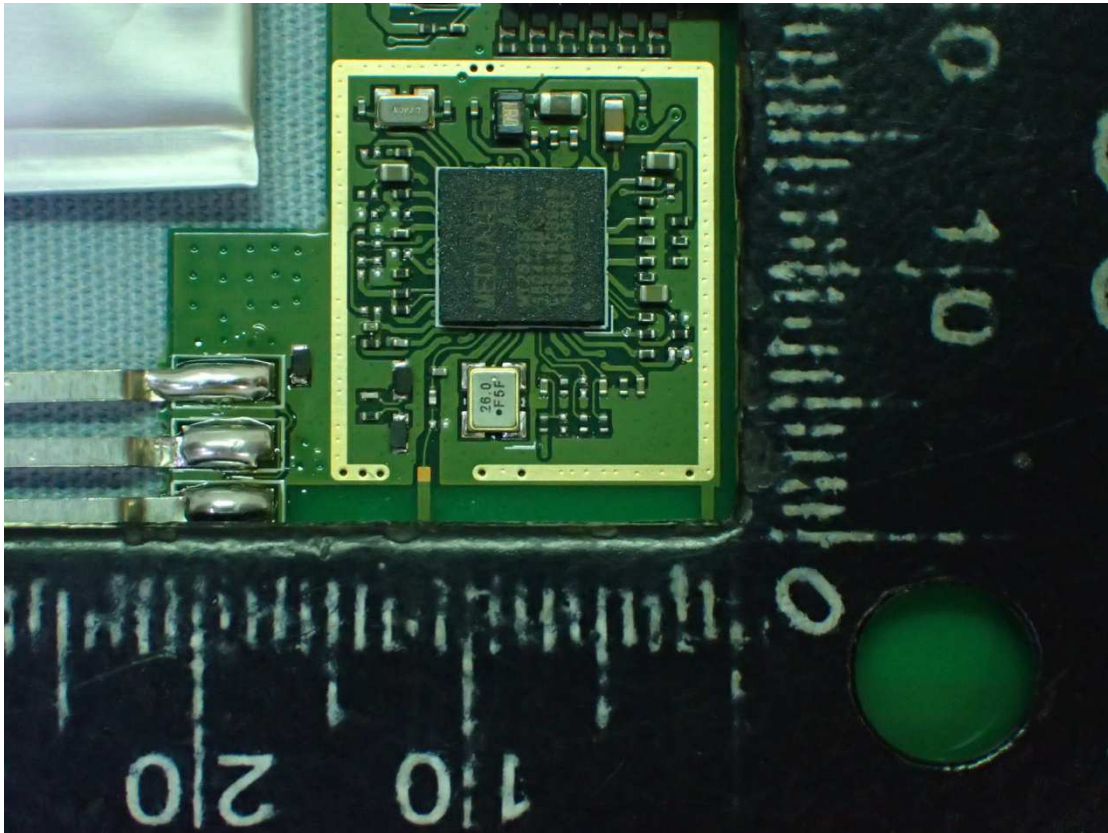
Figure 13 Internal View (RF Chip)
