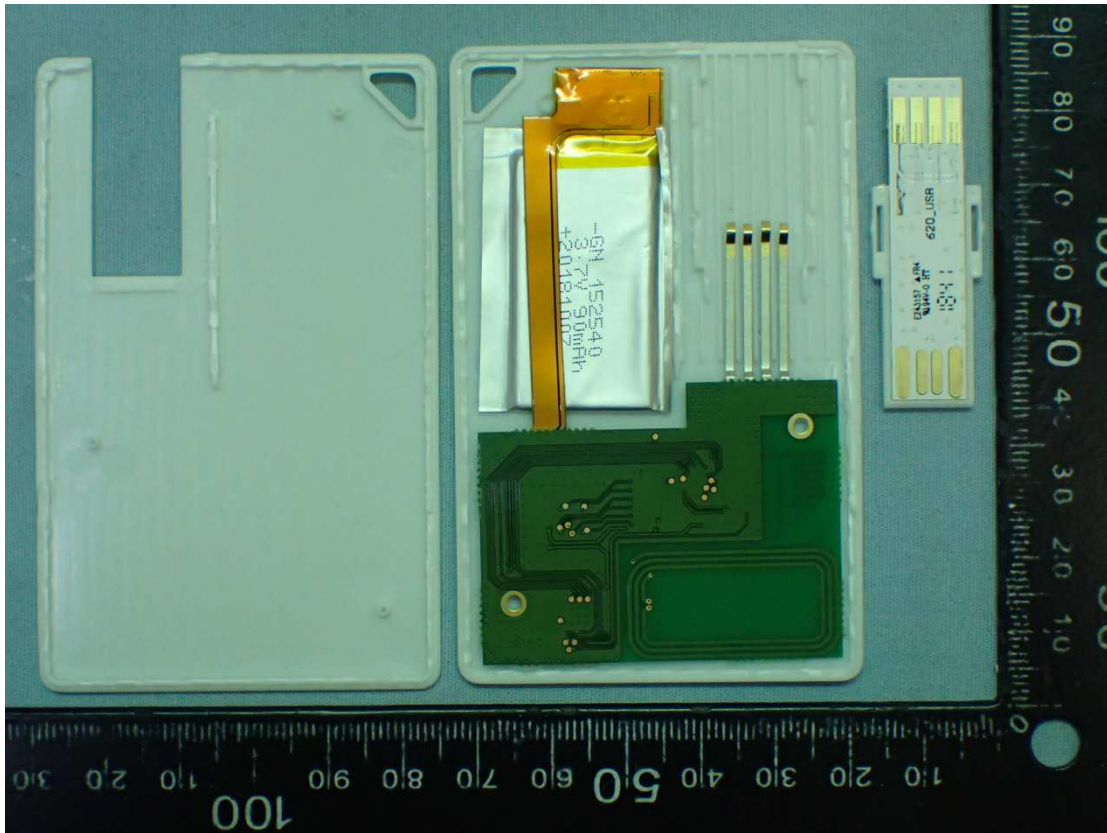
Figure 10 Internal View (Removed Main Board)
