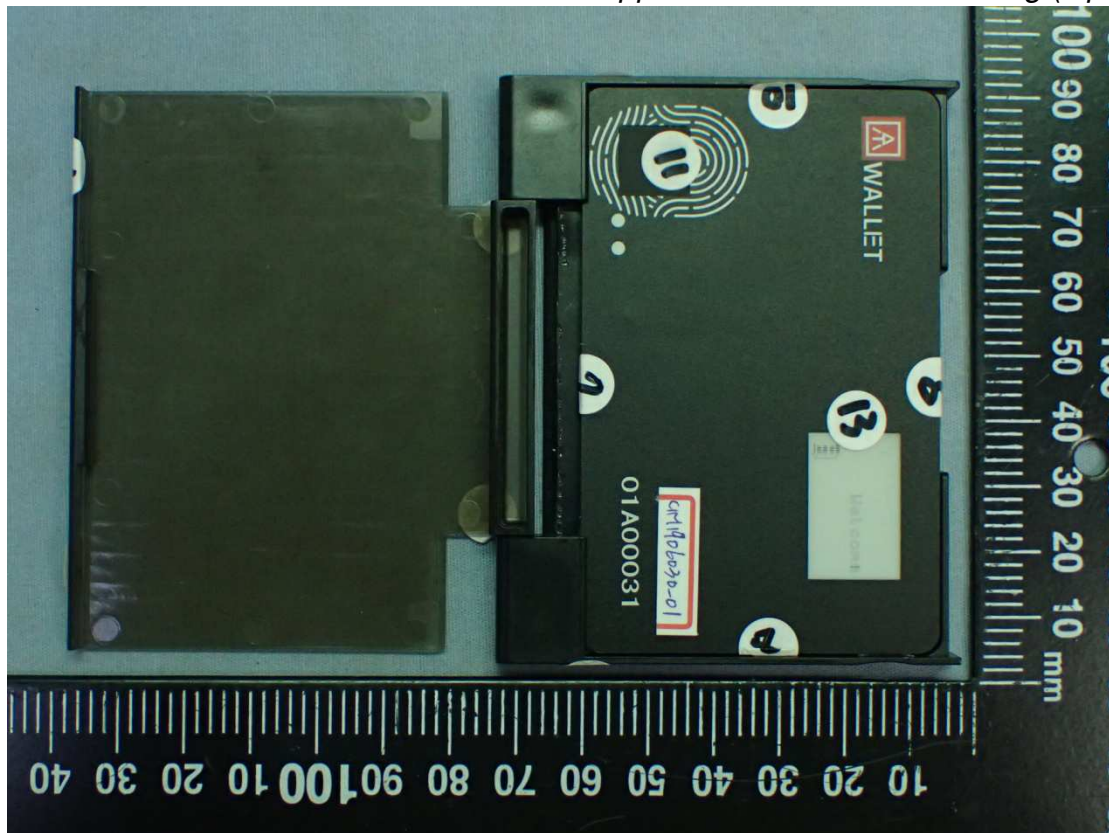
Figure 7 General Appearance With USB Docking (Open Case)
