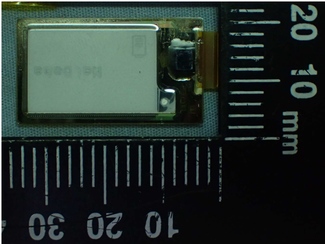
Figure 23 Internal View (E-ink Display, Front View)
