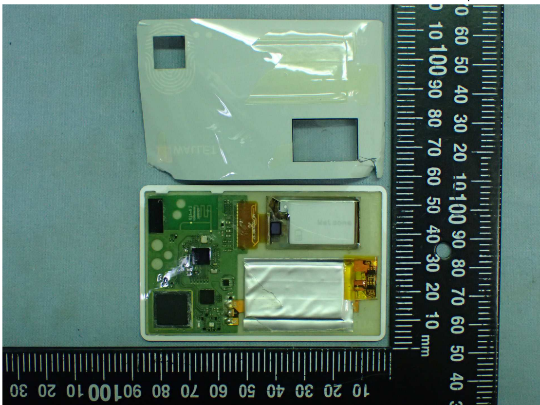
Figure 18 Internal View (Removed Cover)
