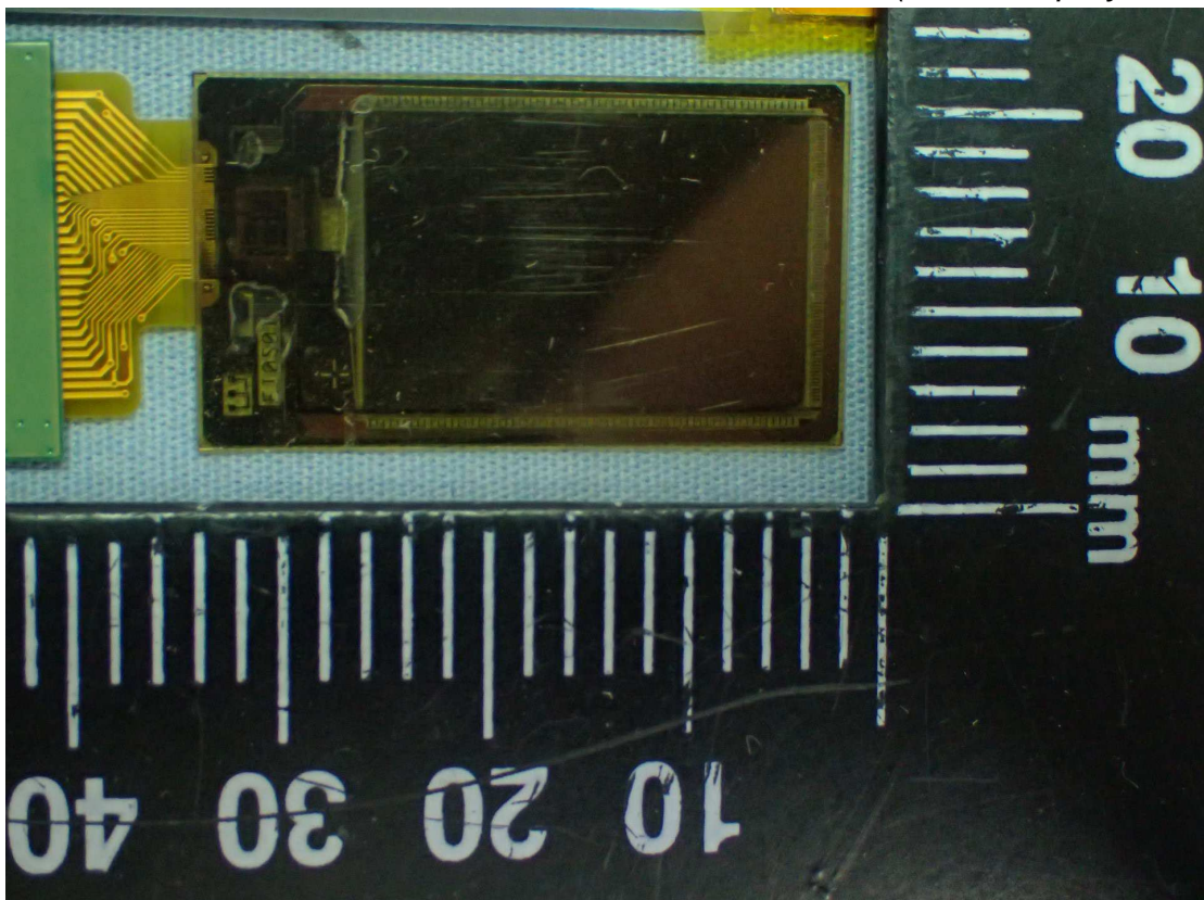
Figure 24 Internal View (E-ink Display, Back View)
