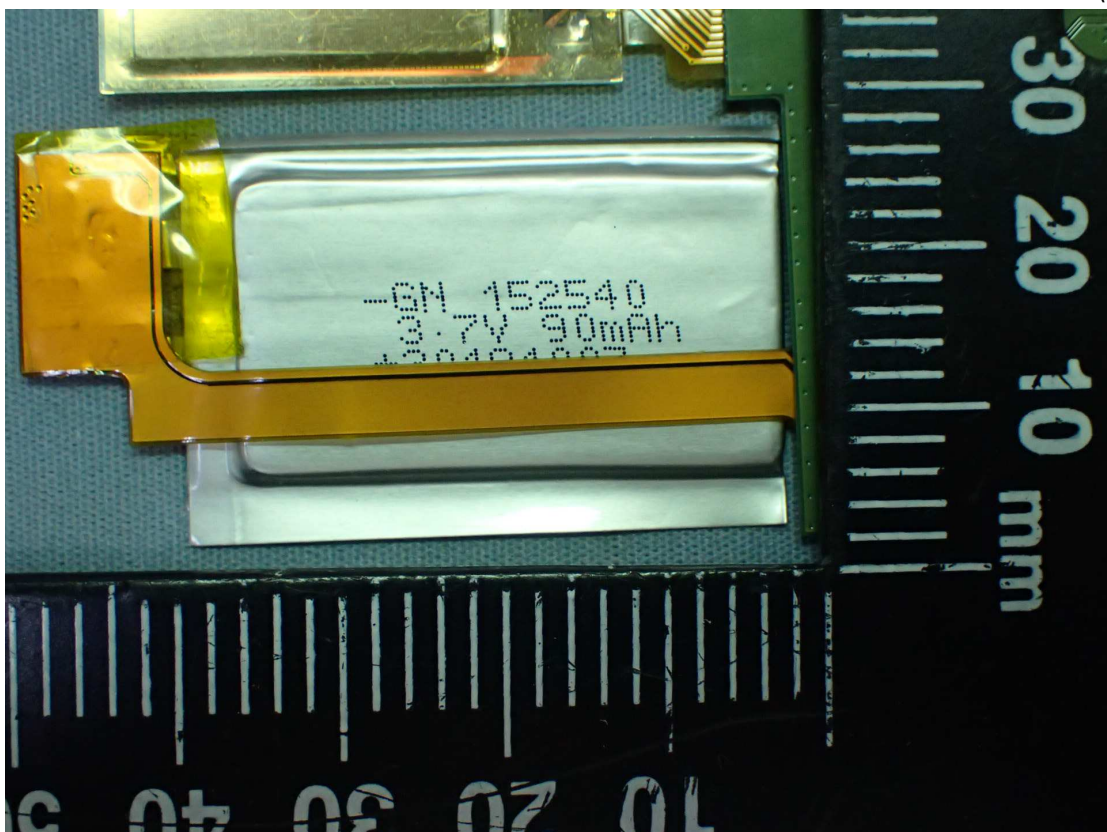
Figure 22 Internal View (Battery)
