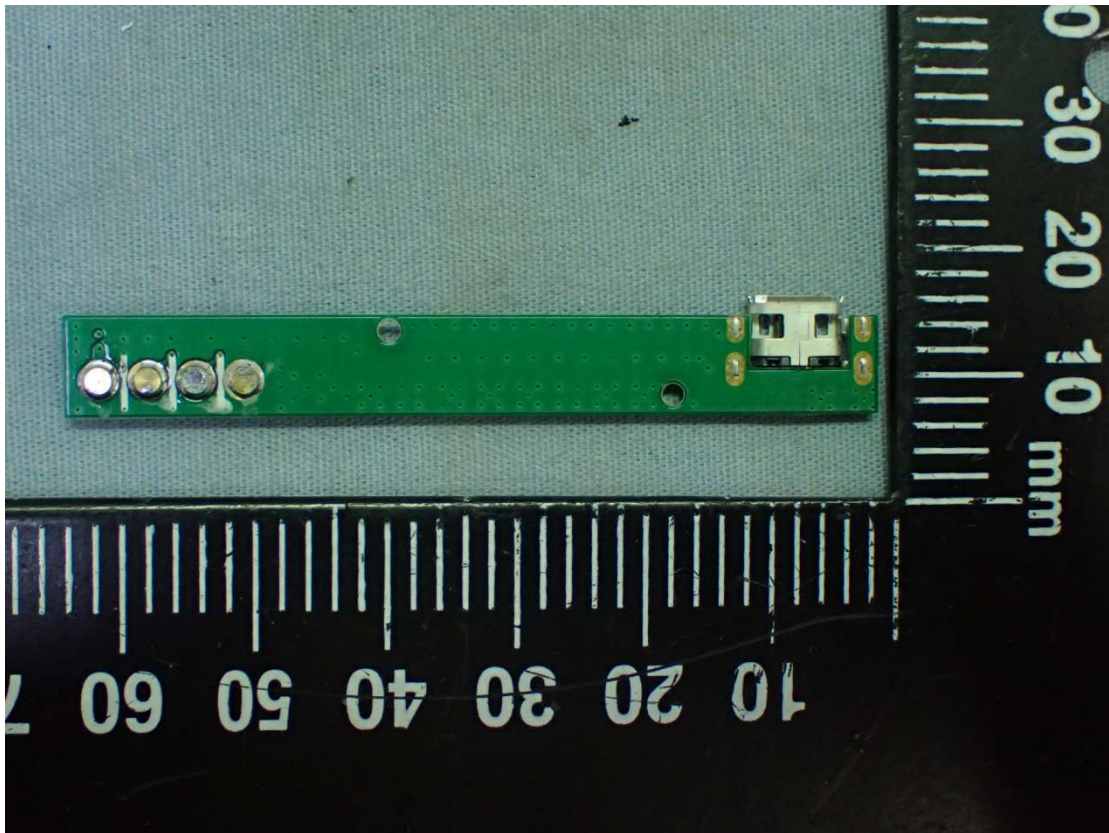
Figure 17 USB Docking Internal View (Control Board, Back View)
