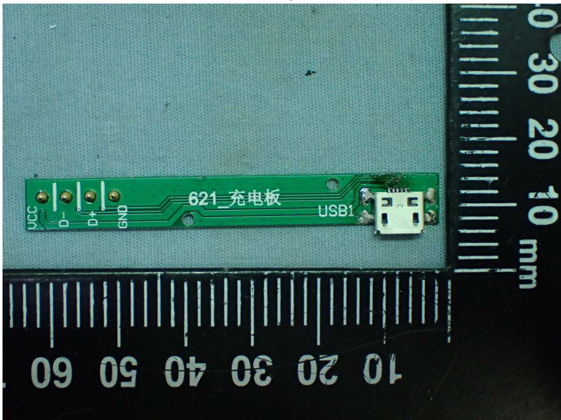
USB Docking Internal View (Control Board, Front View)
