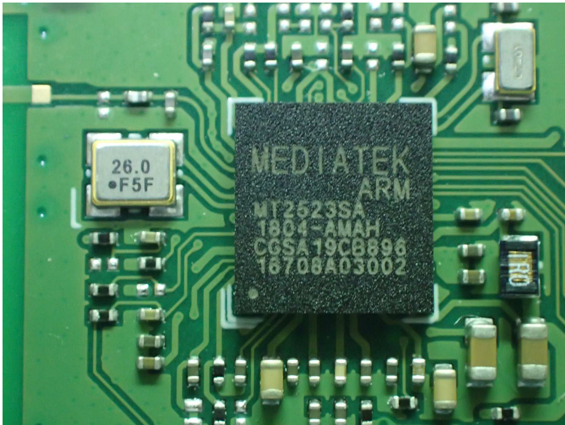
Figure 21 Internal View (RF Chip)
