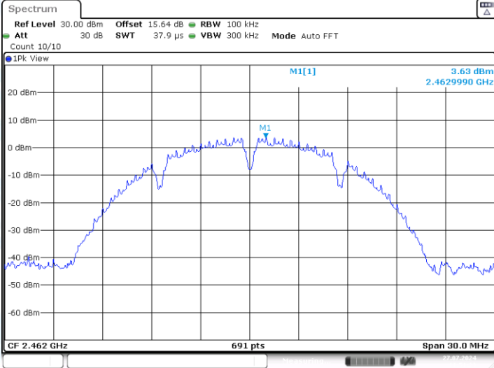
11B-CDD-Ant1-2462-0~Reference-PASS
