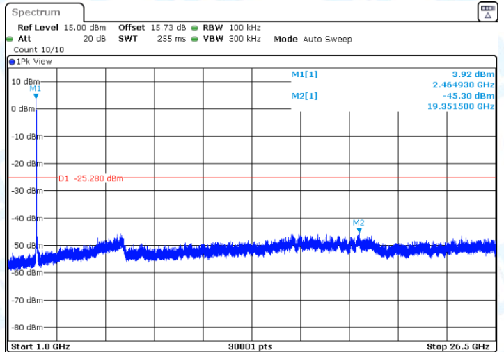
11G-Ant2-2462-0~Reference-PASS
