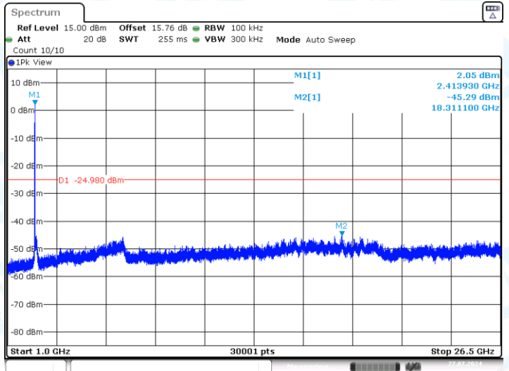
11G-Ant2-2412-0~Reference-PASS
