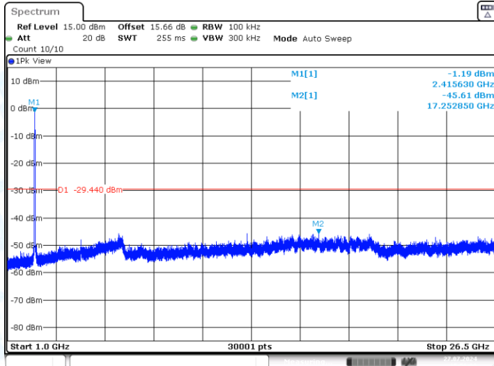
11N40-CDD-Ant1-2422-0~Reference-PASS
