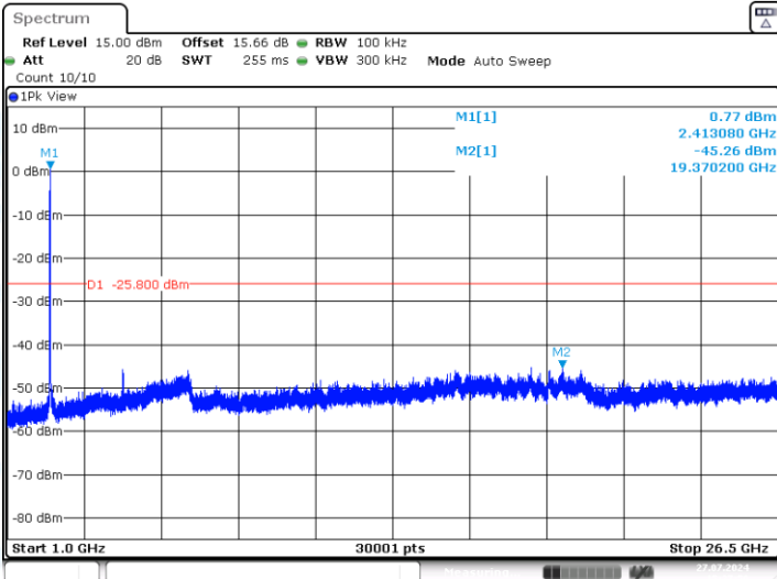
11N20-CDD-Ant1-2412-0~Reference-PASS
