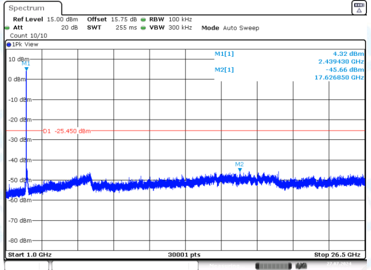
11G-Ant2-2437-0~Reference-PASS
