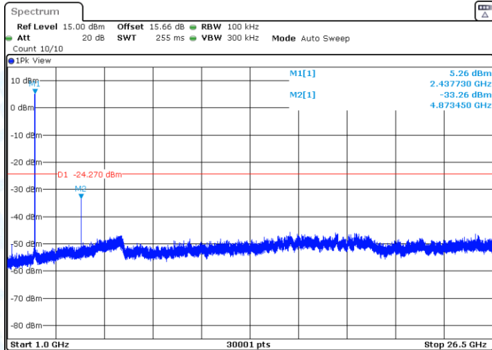
11B-Ant1-2437-0~Reference-PASS
