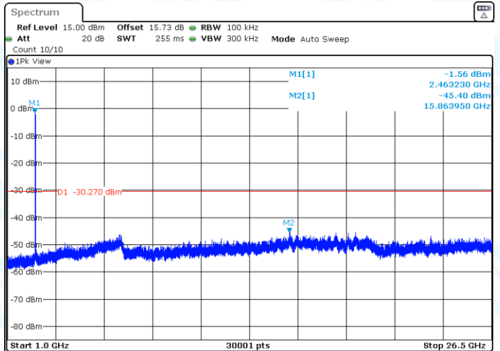
11N20-CDD-Ant2-2462-0~Reference-PASS
