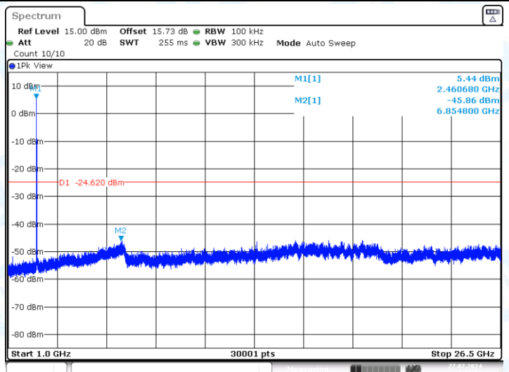
11B-Ant2-2462-0~Reference-PASS
