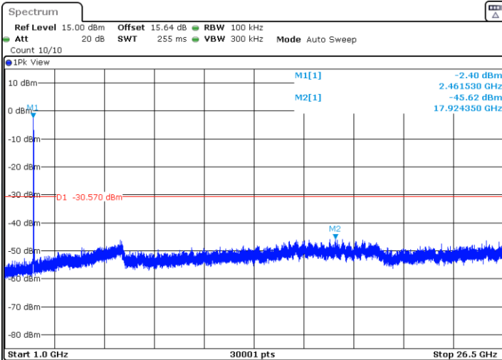
11N20-CDD-Ant1-2462-0~Reference-PASS
