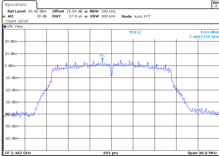
11G-Ant1-2462-0~Reference-PASS
