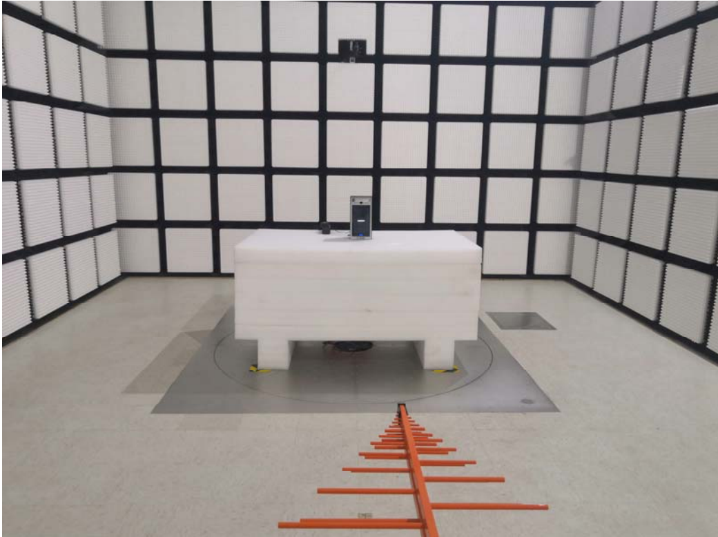
Radiated EmissionsAbove 30 MHz View
