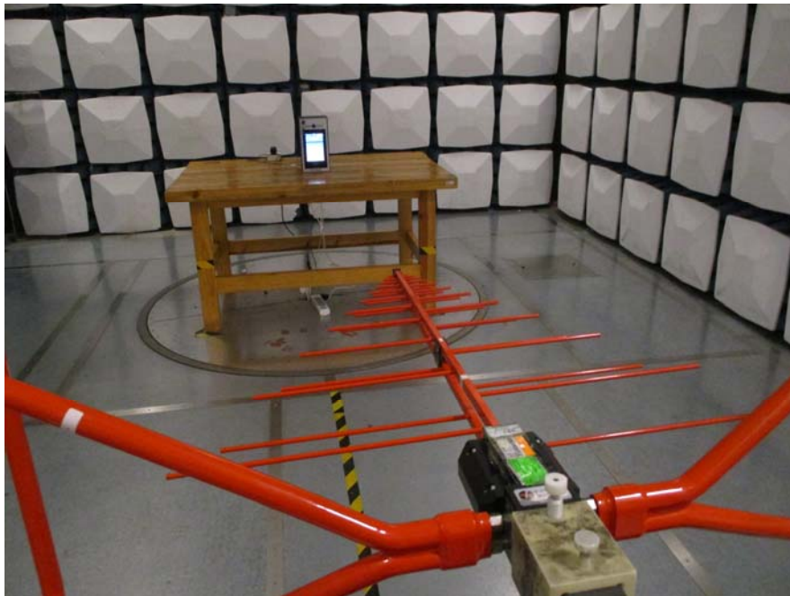
Radiated Emission- Adapter View (30 MHz ~1 GHz)
