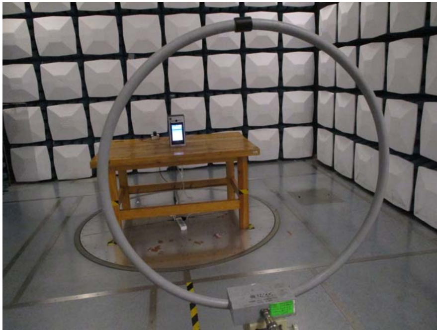
Radiated Emission-Adapter View (9 kHz~30 MHz)
