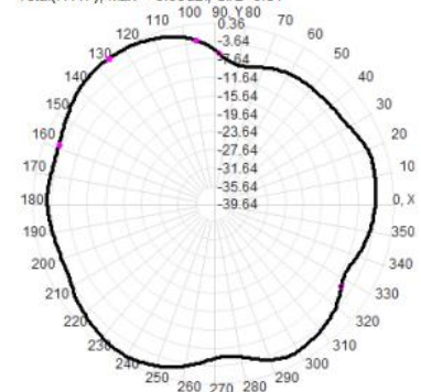
Total(H-XY), Max= -0.00dBi, CirD=8.51
