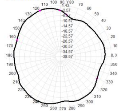
Total(H-XY), Max= 0.78dBi, CirD=8.58
