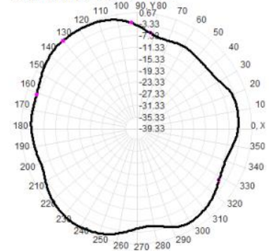
Total(H-XY), Max= 0.25dBi, CirD=7.57
