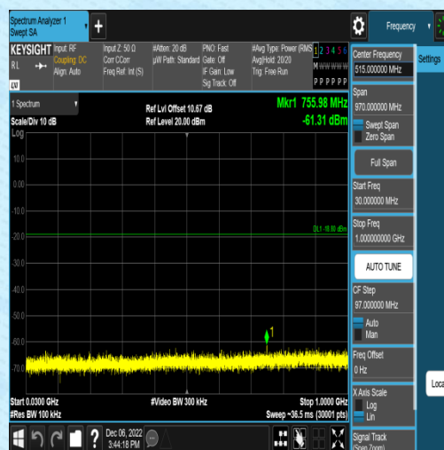
BLE_1M-Ant1-2440-0~Reference
