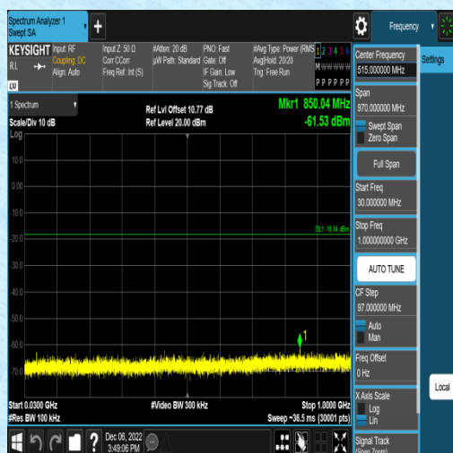
BLE_1M-Ant1-2480-0~Reference
