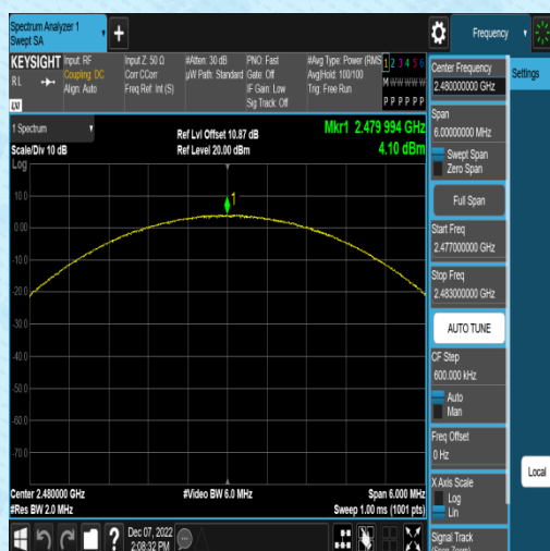
3DH5-Ant1-2480
