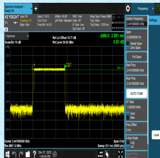
2DH3-Ant1-Hop
