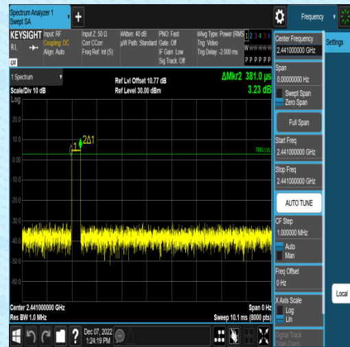
2DH5-Ant1-Hop
