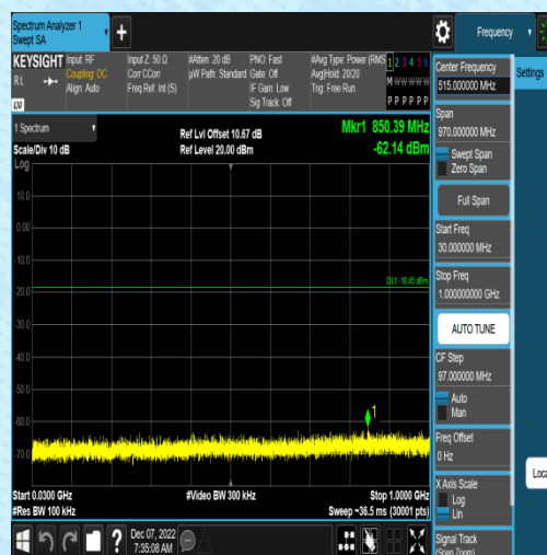
2DH5-Ant1-2402-0~Reference
