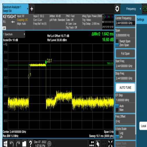
3DH3-Ant1-Hop
