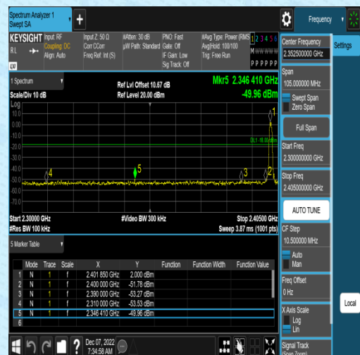
2DH5-Ant1-Low-2402
