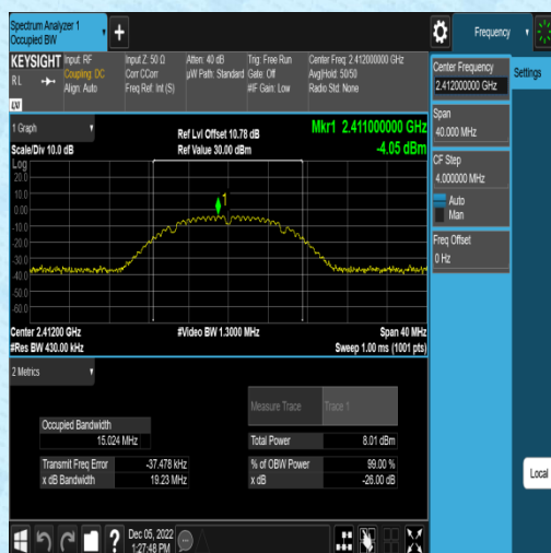
11B-Ant2-2462
