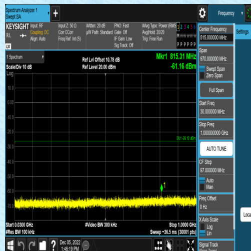
11N20SISO-Ant2-2437-0~Reference--7.08
