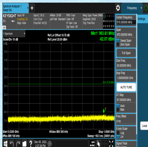
11N40MIMO-Ant1-2437-0~Reference--5.47
