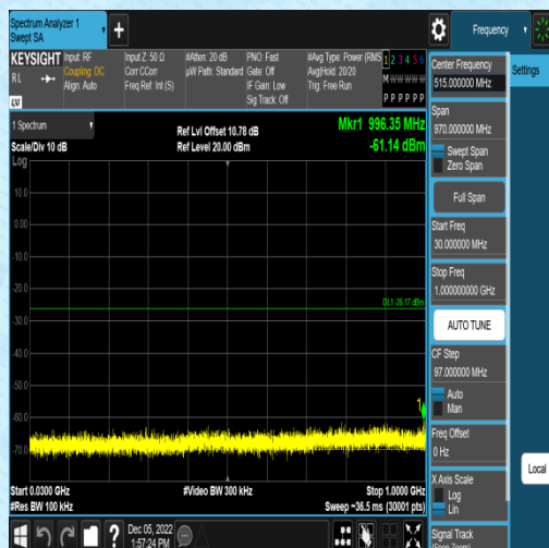
11N40SISO-Ant2-2437-0~Reference--7.81
