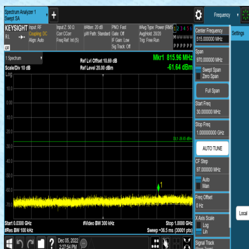
11N40MIMO-Ant1-2422-0~Reference--4.83
