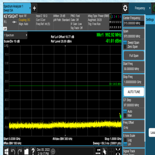
11N20MIMO-Ant2-2437-0~Reference--6.73
