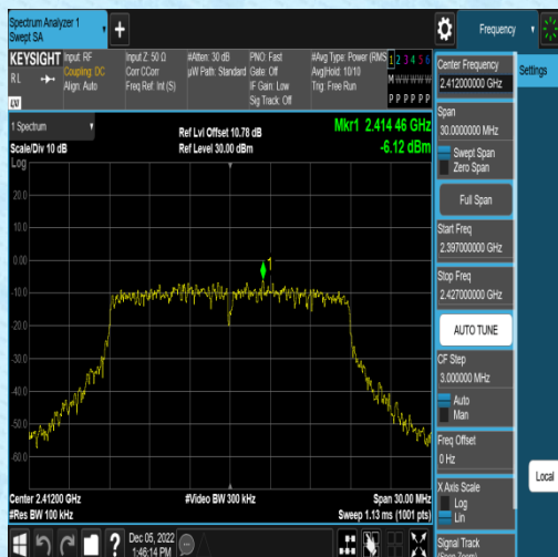
11N20SISO-Ant2-2412-1000~26500~-6.12
