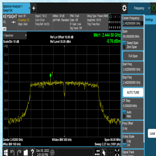
11N40MIMO-Ant1-2452-1000~26500--5.76
