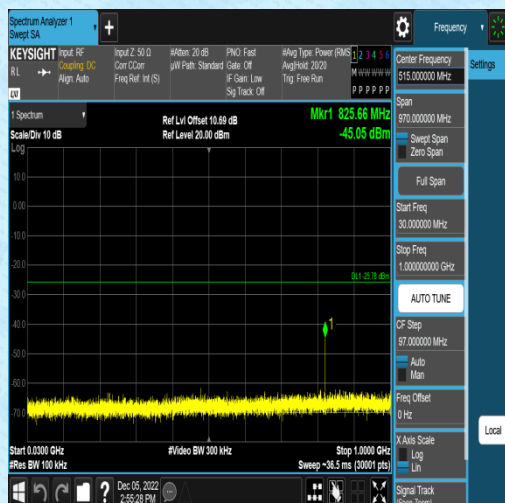
11N40MIMO-Ant2-2452-30~1000--5.78
