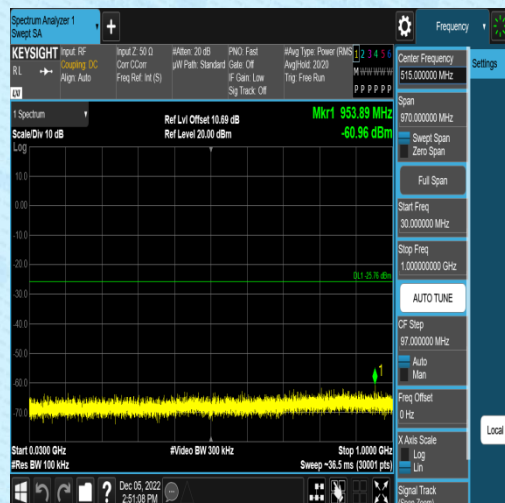
11N40MIMO-Ant2-2452-0~Reference--5.78
