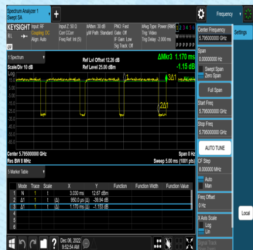
NTNV-11AC40SISO-Ant2-5795
