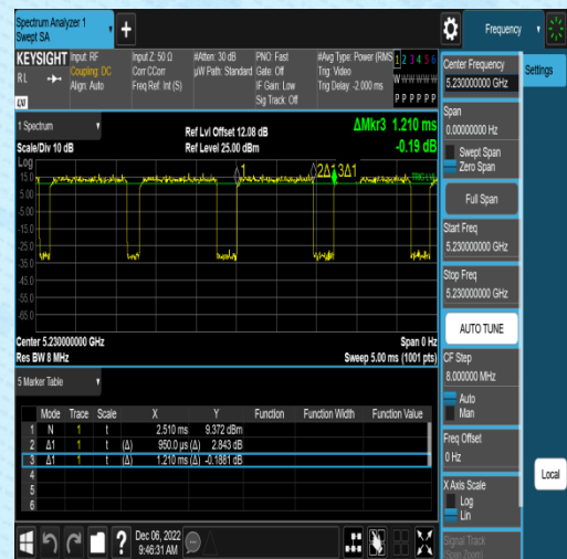
NTNV-11AC40SISO-Ant2-5230
