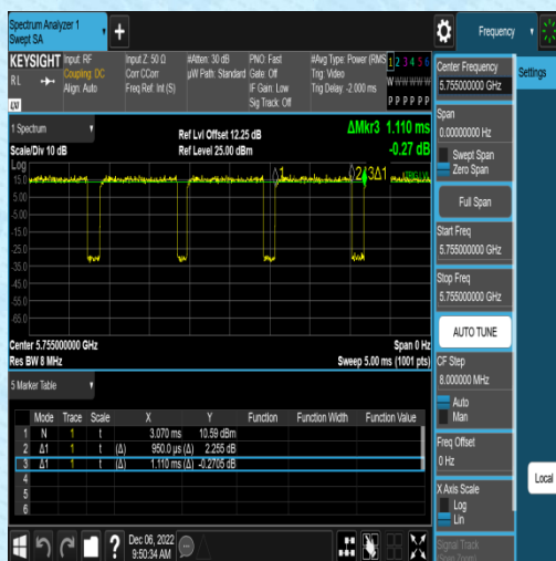
NTNV-11AC40SISO-Ant2-5755
