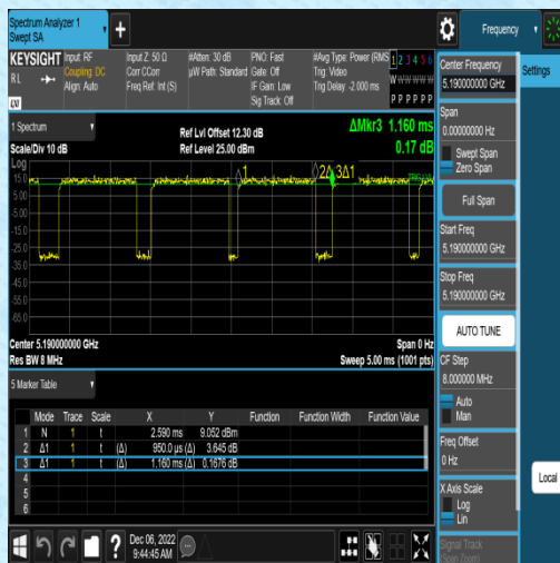
NTNV-11AC40SISO-Ant2-5190
