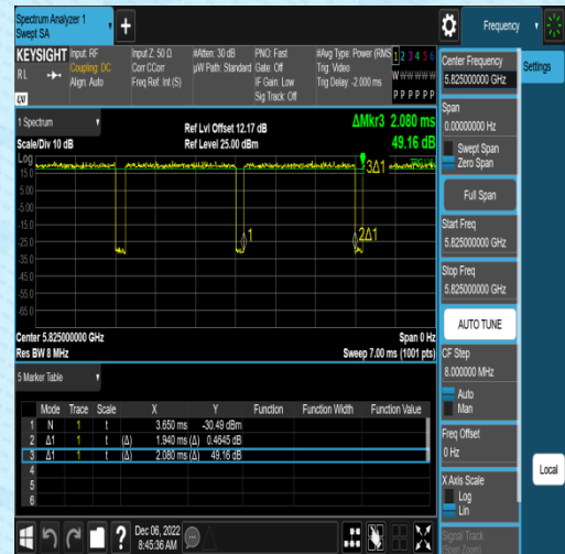
NTNV-11AC40SISO-Ant2-5230
