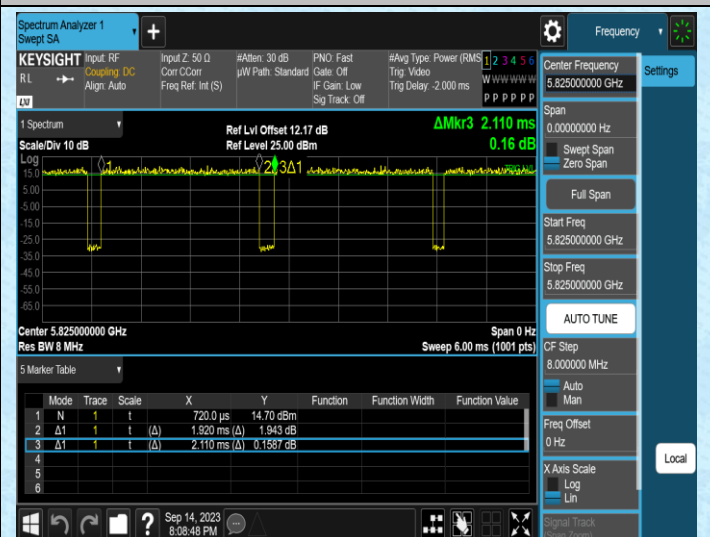
NTNV-11N20SISO-Ant2-5825
