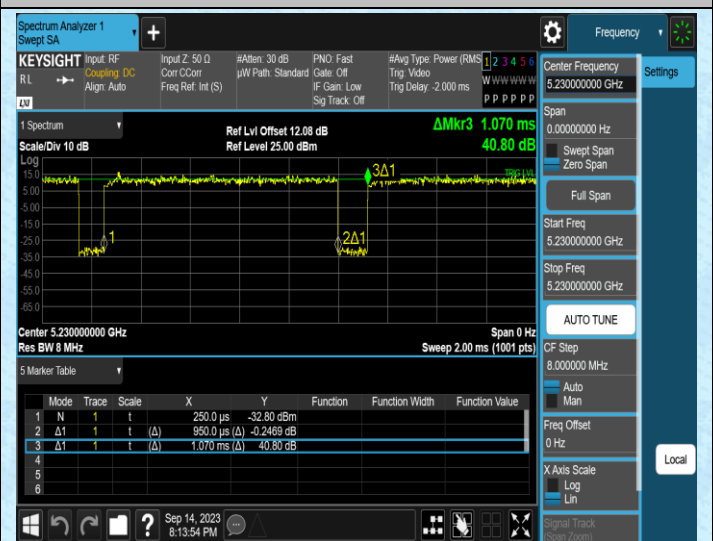
NTNV-11N40SISO-Ant2-5230
