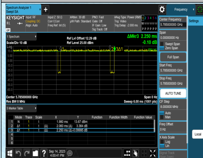
NTNV-11A-Ant1-5785
