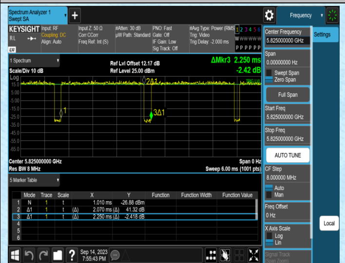
NTNV-11A-Ant2-5825
