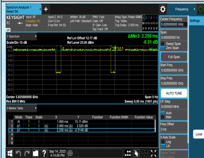
NTNV-11A-Ant1-5825
