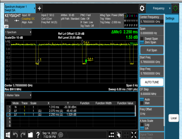
NTNV-11A-Ant2-5785
