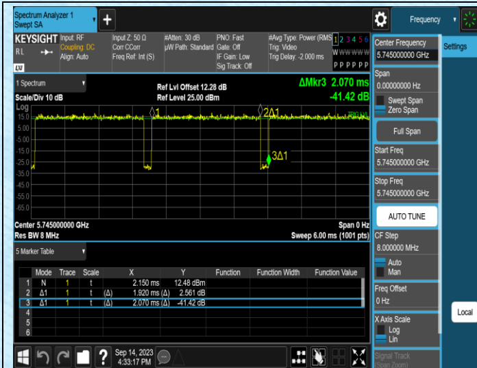
NTNV-11N20SISO-Ant1-5745
