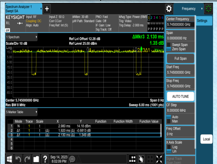
NTNV-11N20SISO-Ant2-5745
