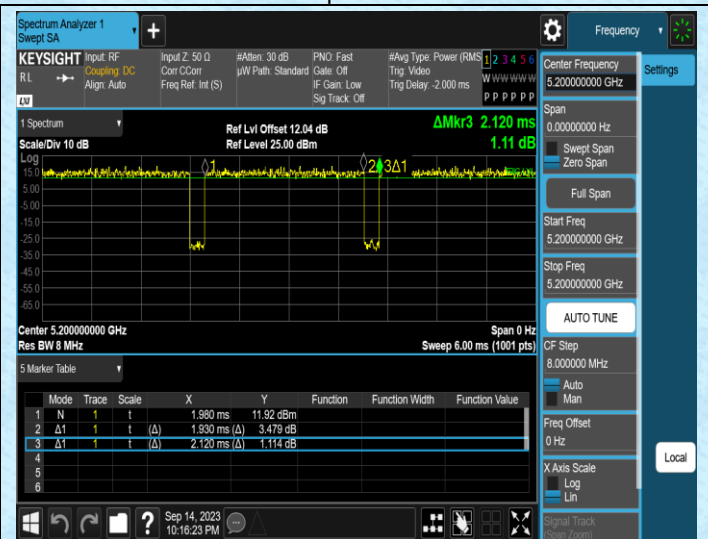
NTNV-11AC20MIMO-Ant2-5200
