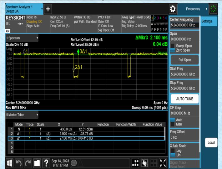
NTNV-11N20MIMO-Ant2-5240
