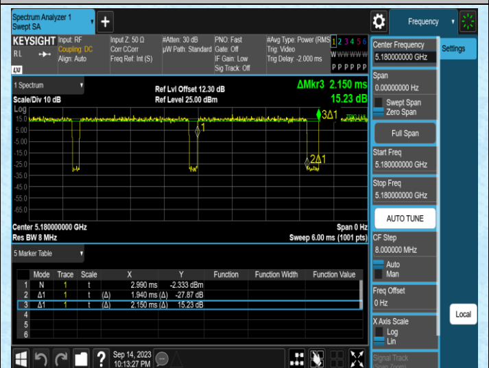
NTNV-11AC20MIMO-Ant2-5180
