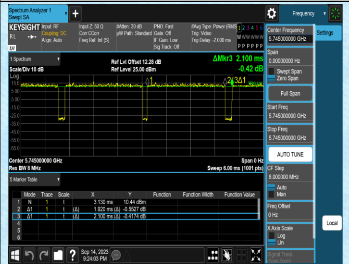
NTNV-11N20MIMO-Ant2-5745
