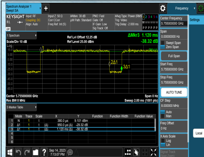
NTNV-11AC40SISO-Ant1-5755
