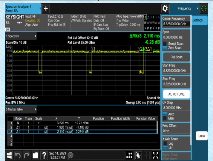
NTNV-11N20MIMO-Ant2-5825
