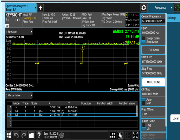
NTNV-11AC20SISO-Ant1-5745
