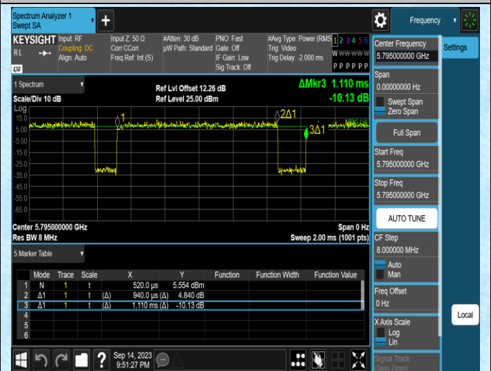
NTNV-11N40MIMO-Ant2-5795
