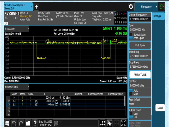
NTNV-11N40MIMO-Ant2-5755
