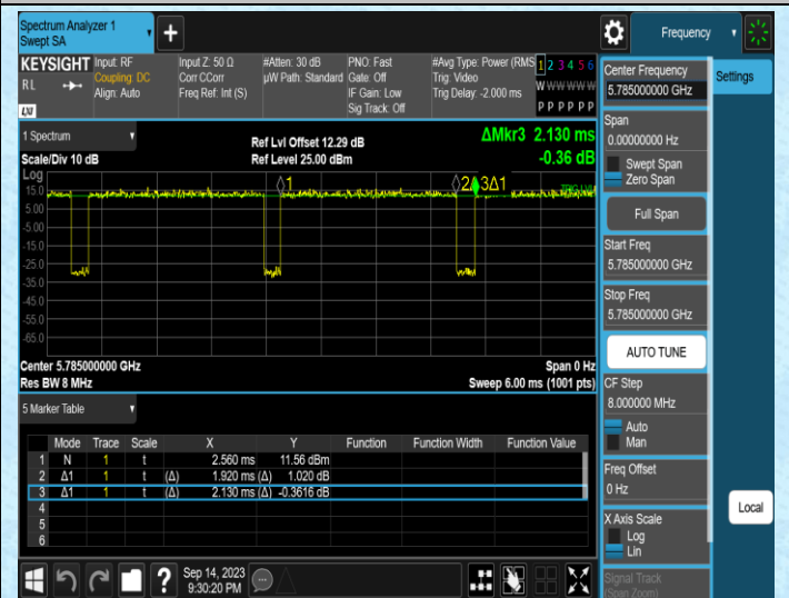
NTNV-11N20MIMO-Ant2-5785
