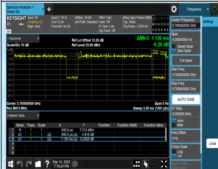
NTNV-11AC40SISO-Ant1-5795
