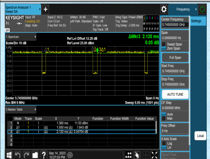
NTNV-11AC20MIMO-Ant2-5745
