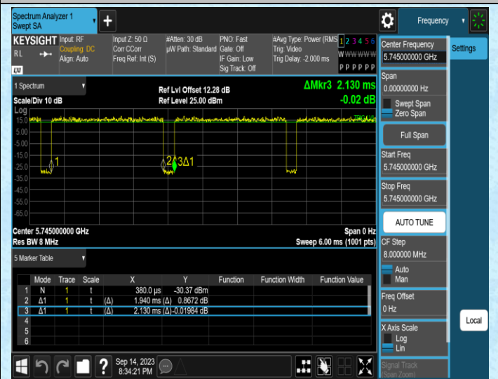
NTNV-11AC20SISO-Ant2-5745
