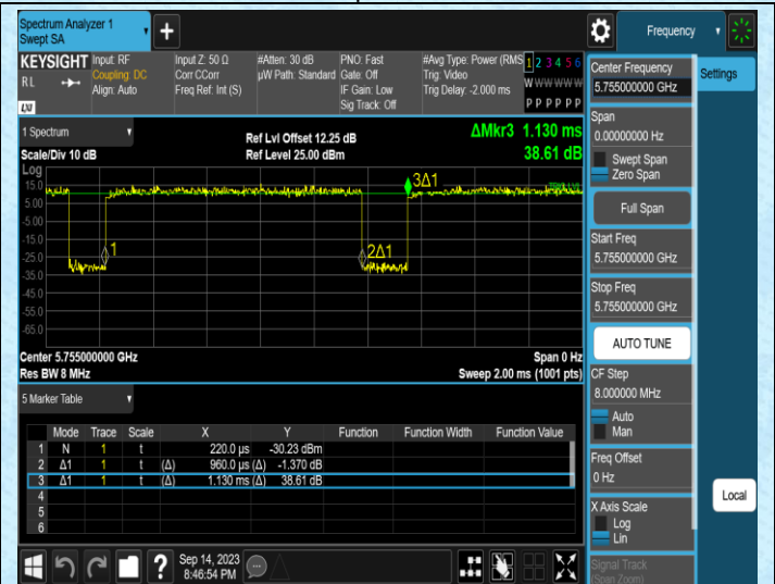
NTNV-11AC40SISO-Ant2-5755
