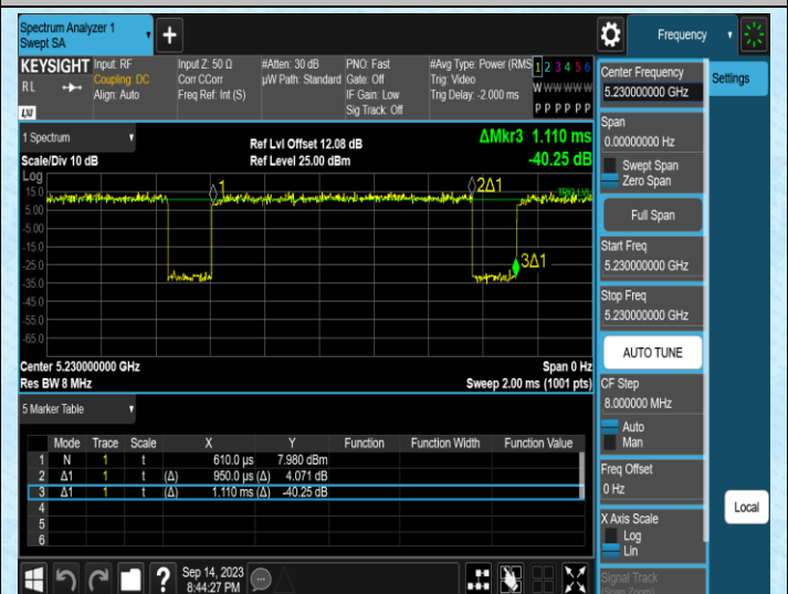
NTNV-11AC40SISO-Ant2-5230
