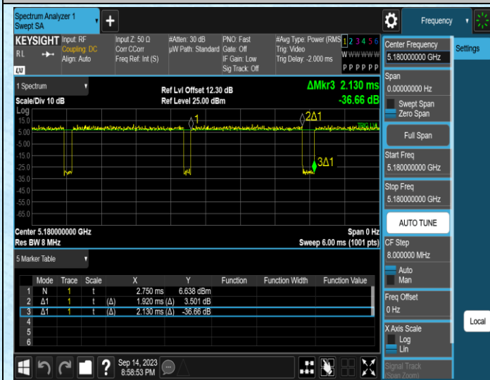
NTNV-11N20MIMO-Ant1-5180
