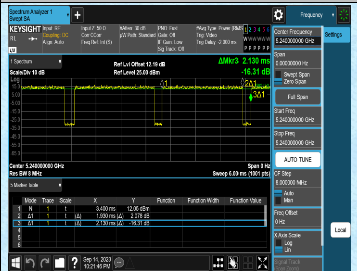
NTNV-11AC20MIMO-Ant2-5240
