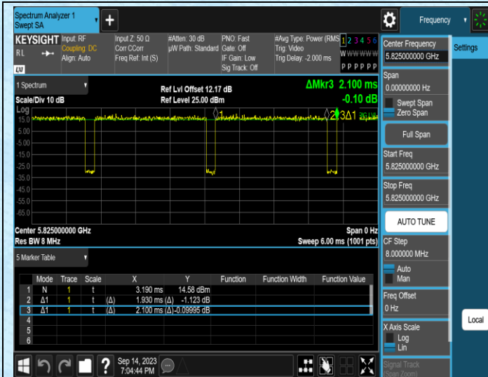
NTNV-11AC20SISO-Ant1-5825
