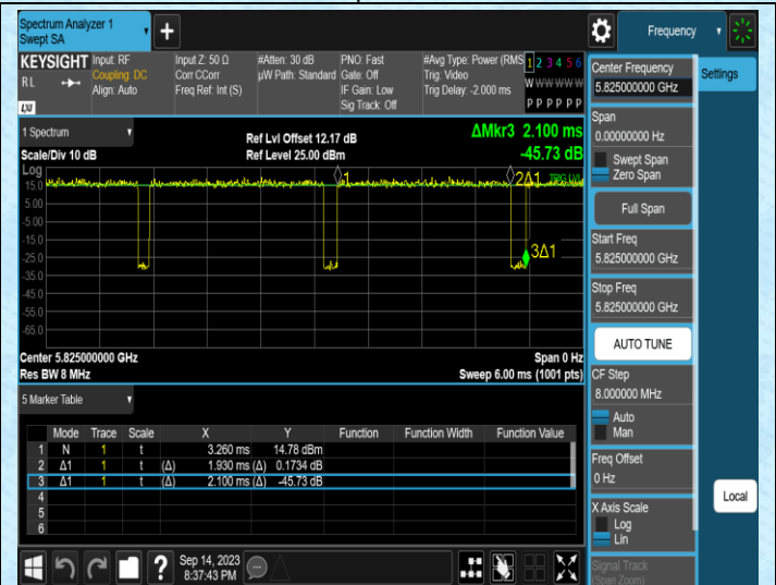
NTNV-11AC20SISO-Ant2-5825
