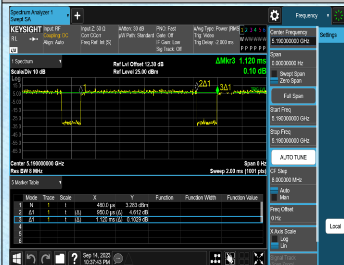
NTNV-11AC40MIMO-Ant1-5190
