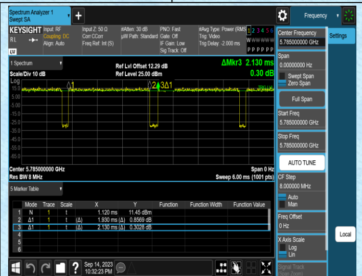
NTNV-11AC20MIMO-Ant2-5785
