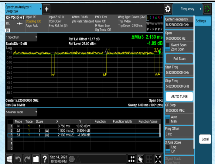
NTNV-11AC20MIMO-Ant2-5825
