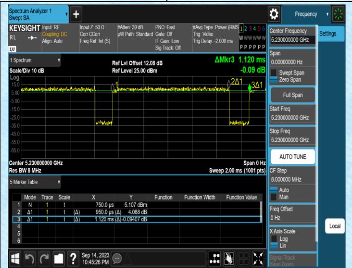
NTNV-11AC40MIMO-Ant2-5230
