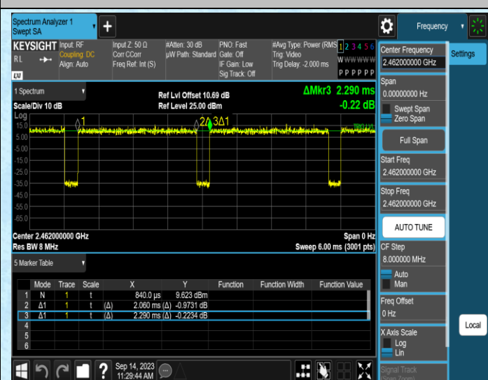
NTNV-11G-Ant2-2462
