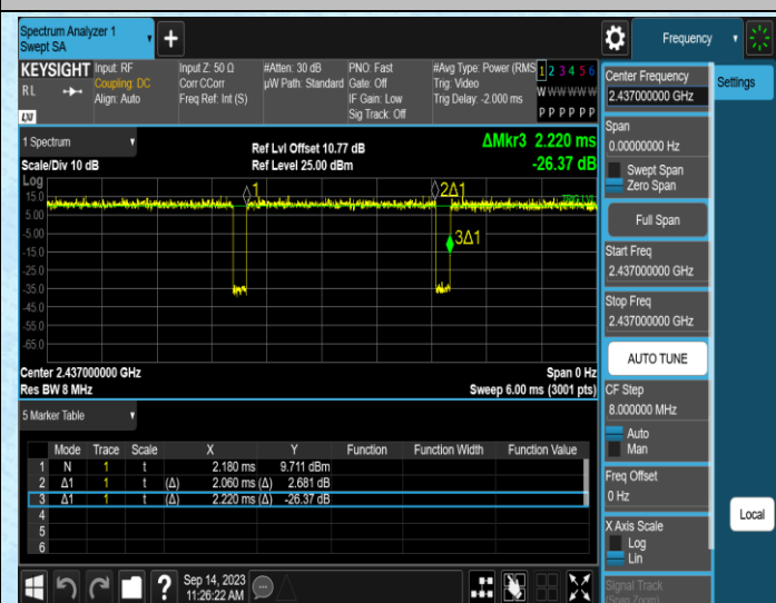
NTNV-11G-Ant2-2437
