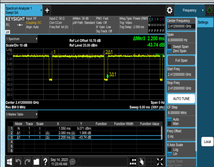
NTNV-11G-Ant2-2412
