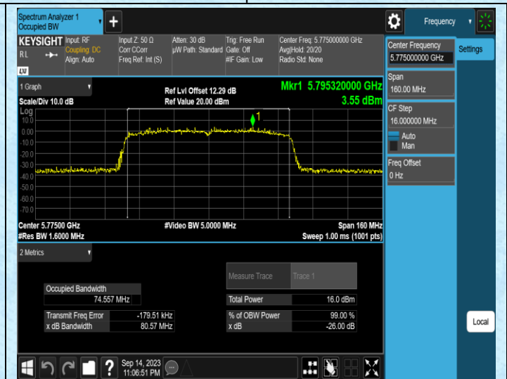
11AC80MIMO-Ant2-5775
