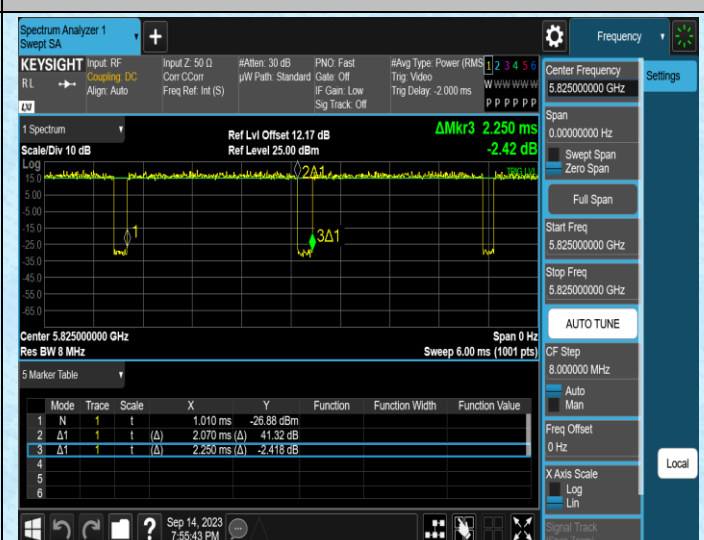
NTNV-11A-Ant2-5825
