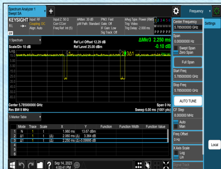
NTNV-11A-Ant1-5785
