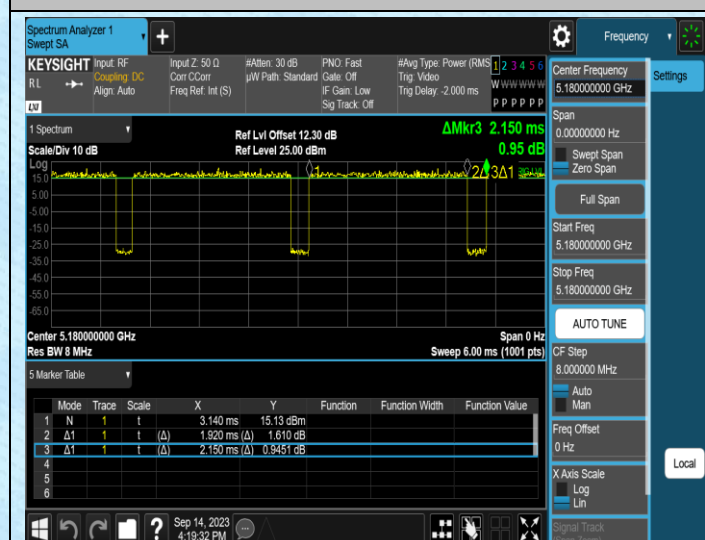
NTNV-11N20SISO-Ant1-5180
