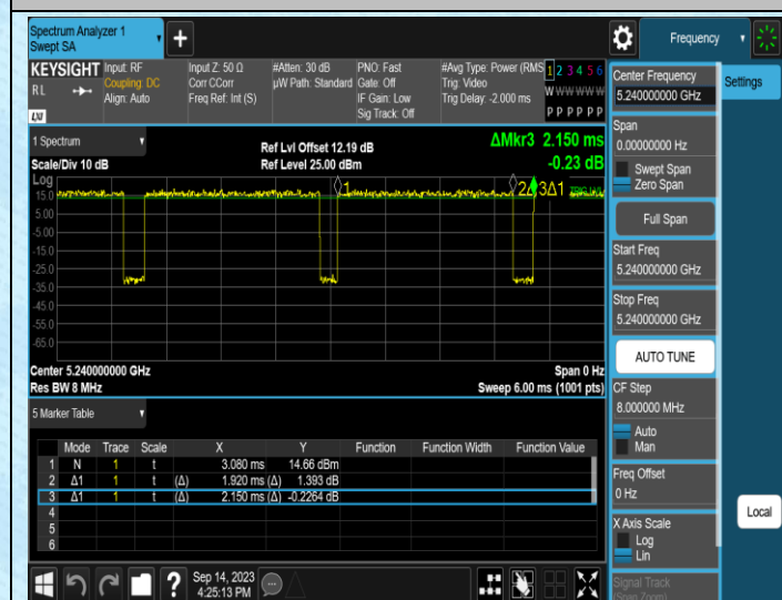
NTNV-11N20SISO-Ant1-5240
