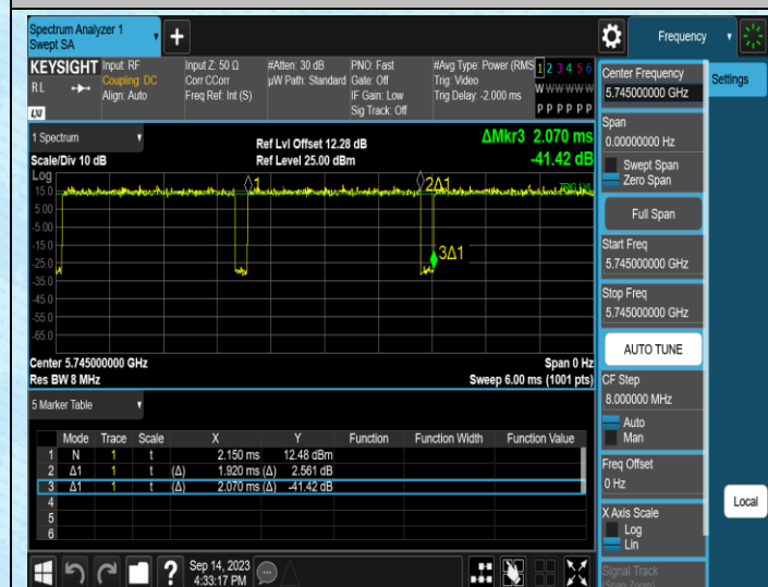
NTNV-11N20SISO-Ant1-5745
