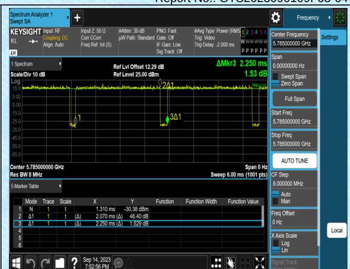
NTNV-11A-Ant2-5785
