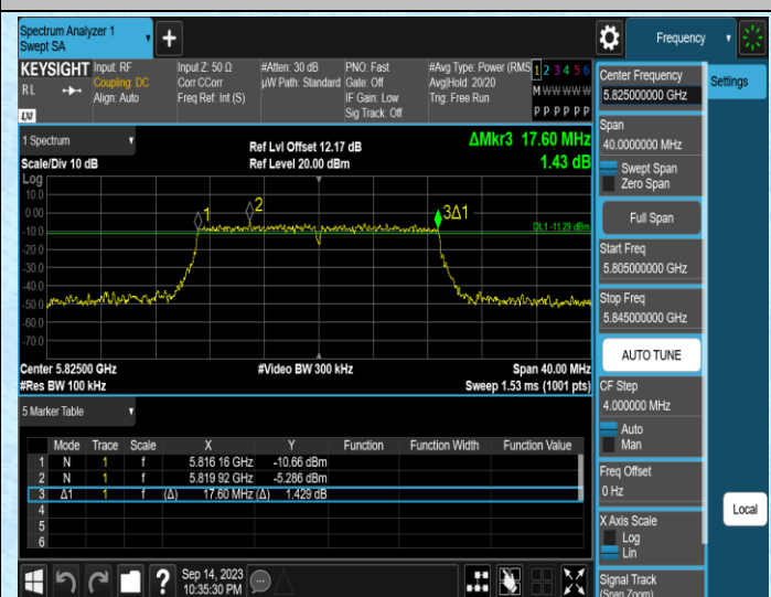
11AC20MIMO-Ant2-5825
