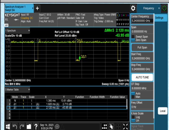
NTNV-11N20SISO-Ant2-5240
