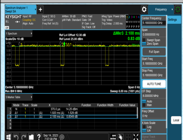
NTNV-11N20SISO-Ant2-5180
