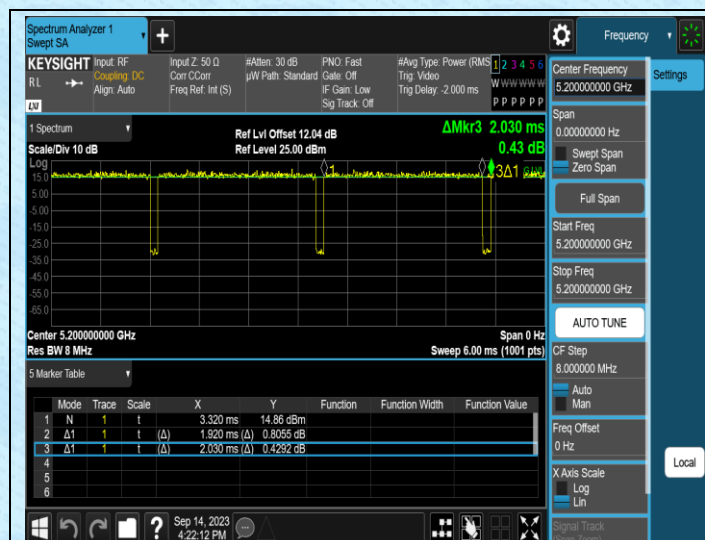
NTNV-11N20SISO-Ant1-5200
