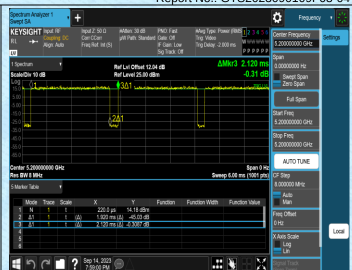
NTNV-11N20SISO-Ant2-5200
