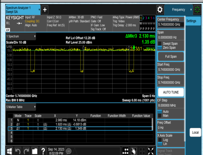
NTNV-11N20SISO-Ant2-5745
