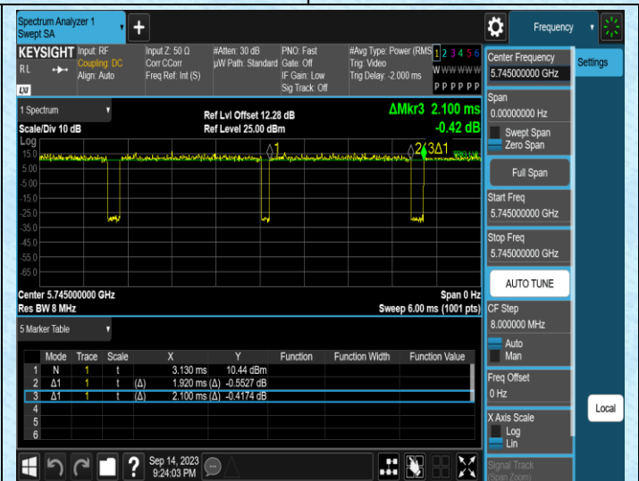
NTNV-11N20MIMO-Ant2-5745
