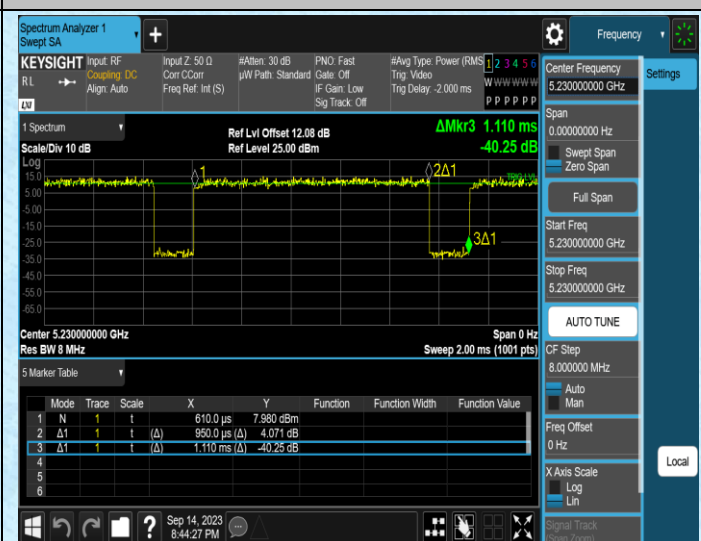
NTNV-11AC40SISO-Ant2-5230
