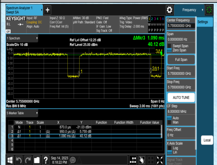
NTNV-11N40SISO-Ant2-5755
