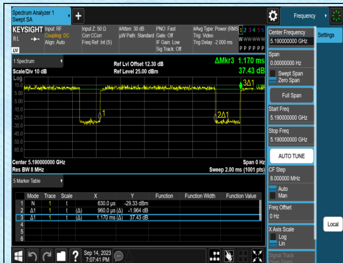
NTNV-11AC40SISO-Ant1-5190
