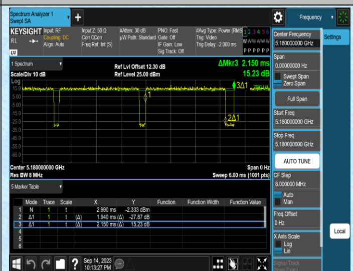
NTNV-11AC20MIMO-Ant2-5180
