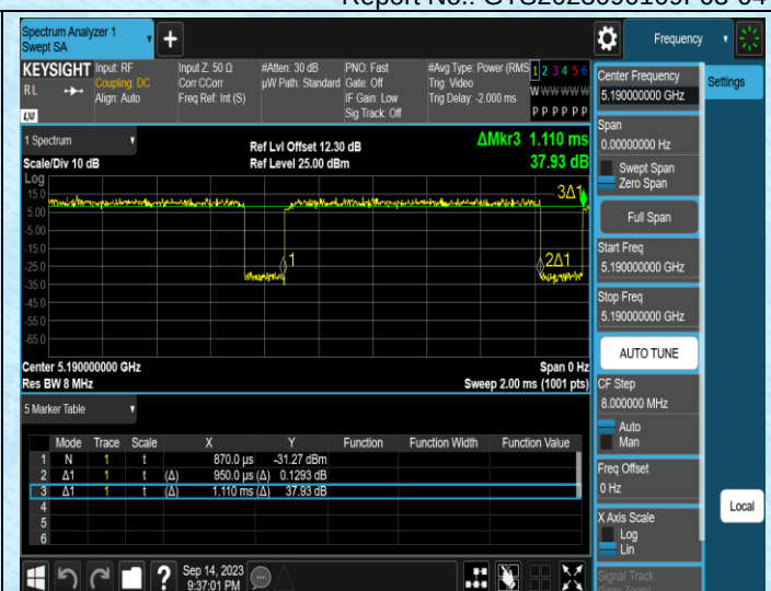
NTNV-11N40MIMO-Ant2-5190
