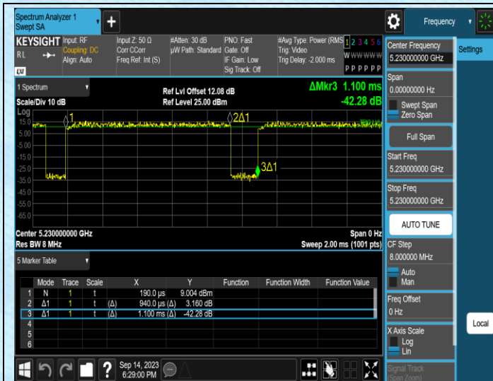
NTNV-11N40SISO-Ant1-5230
