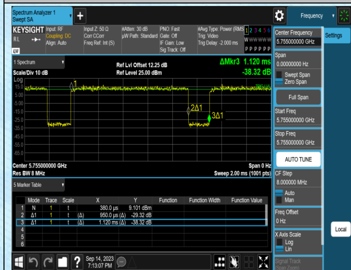
NTNV-11AC40SISO-Ant1-5755
