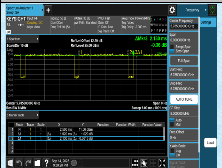
NTNV-11N20MIMO-Ant2-5785
