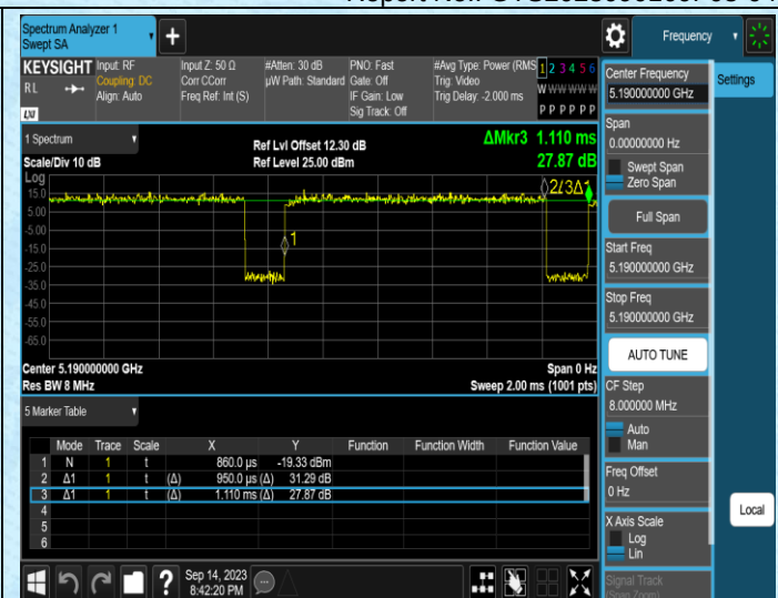
NTNV-11AC40SISO-Ant2-5190
