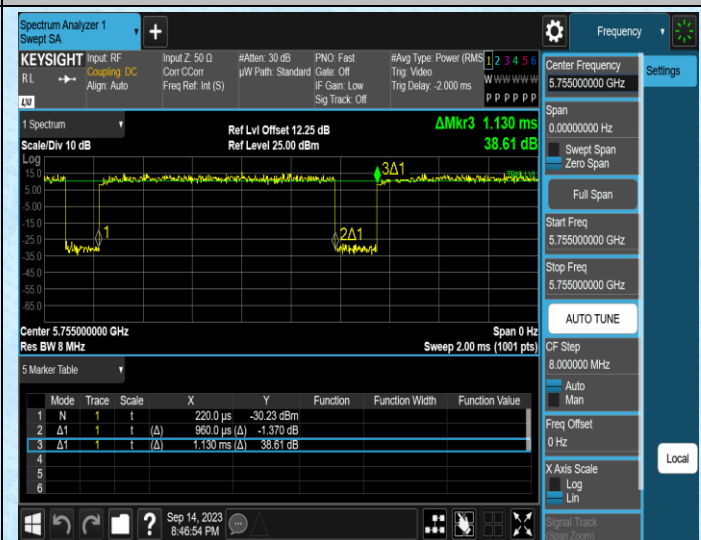
NTNV-11AC40SISO-Ant2-5755
