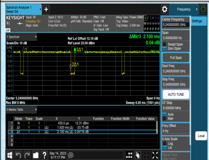
NTNV-11N20MIMO-Ant2-5240
