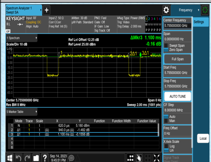
NTNV-11N40MIMO-Ant2-5755
