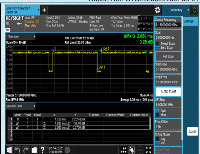
NTNV-11N20MIMO-Ant2-5180
