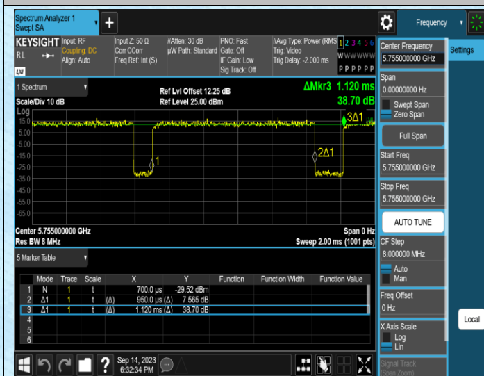
NTNV-11N40SISO-Ant1-5755
