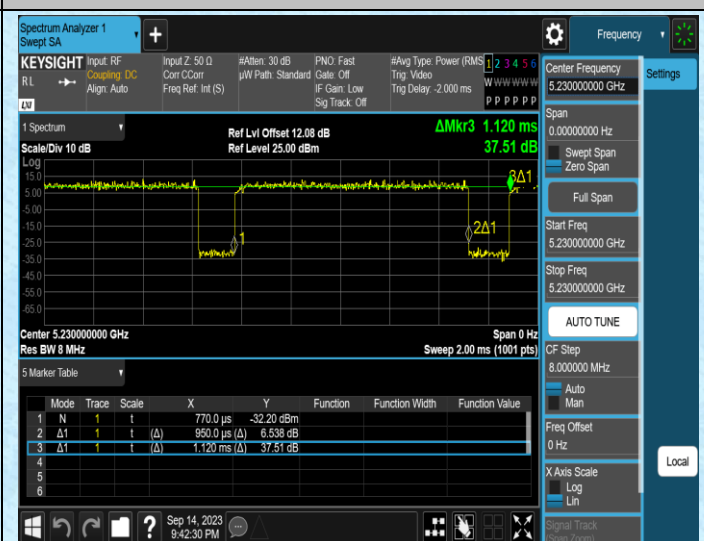
NTNV-11N40MIMO-Ant2-5230
