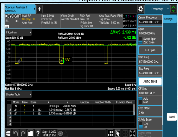
NTNV-11AC20SISO-Ant2-5745
