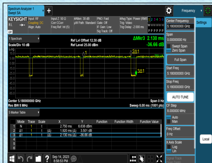
NTNV-11N20MIMO-Ant1-5180
