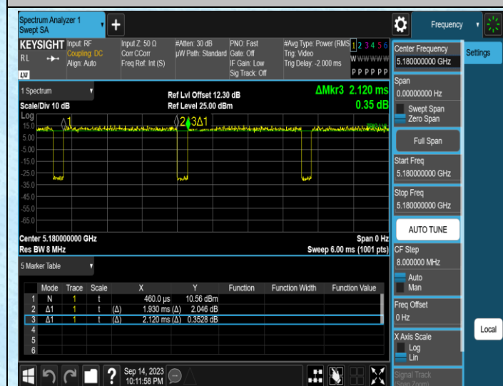
NTNV-11AC20MIMO-Ant1-5180
