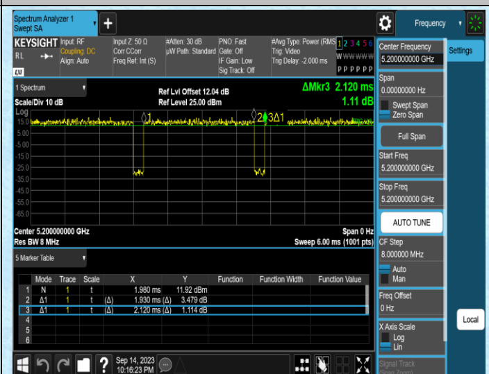
NTNV-11AC20MIMO-Ant2-5200
