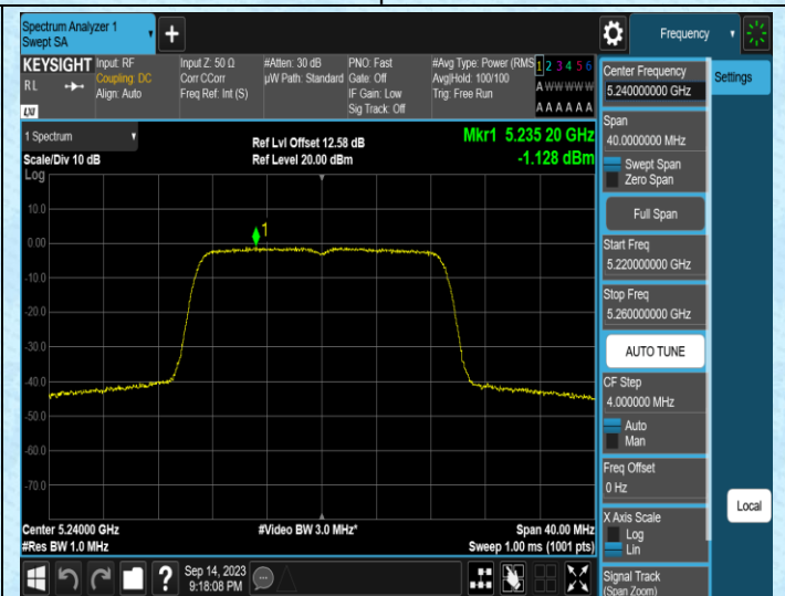
11N20MIMO-Ant2-5240
