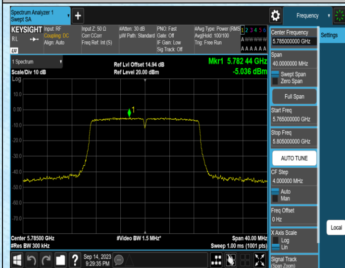
11N20MIMO-Ant1-5785
