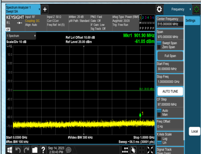
11N20MIMO-Ant2-2462-30~1000
