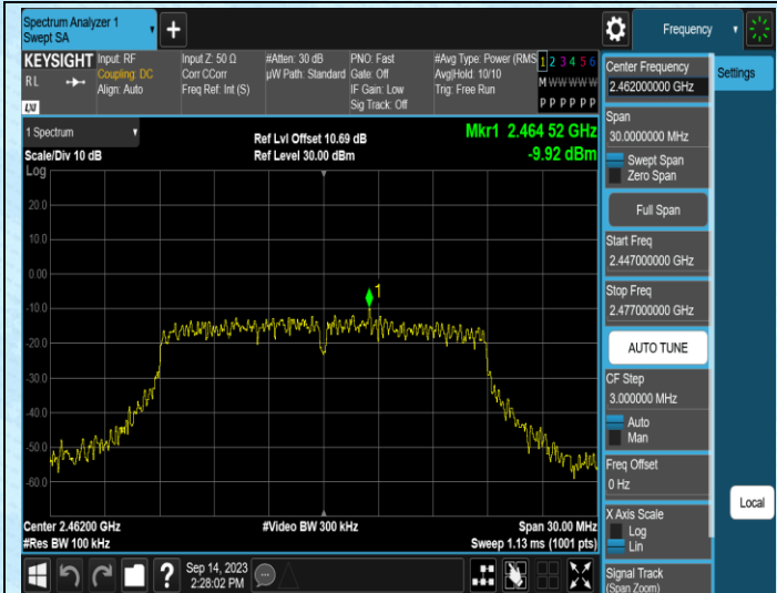
11N20MIMO-Ant1-2462-0~Reference
