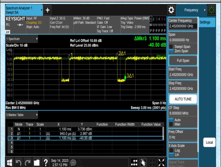
NTNV-11N40MIMO-Ant2-2452
