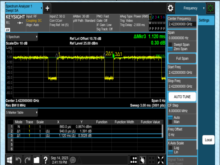
NTNV-11N40MIMO-Ant2-2422
