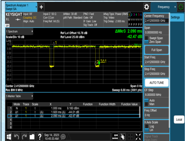
NTNV-11N20SISO-Ant1-2412
