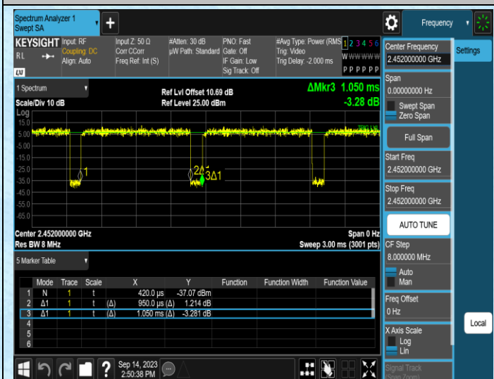
NTNV-11N40MIMO-Ant1-2452
