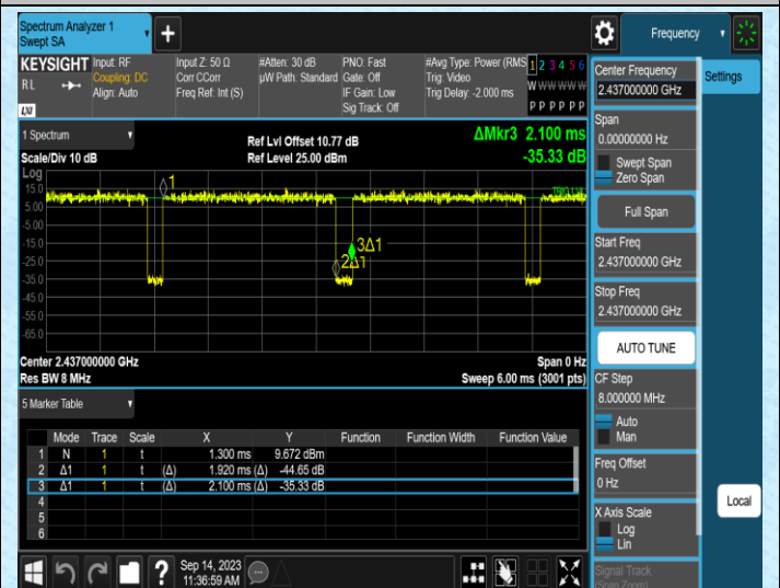
NTNV-11N20SISO-Ant2-2437
