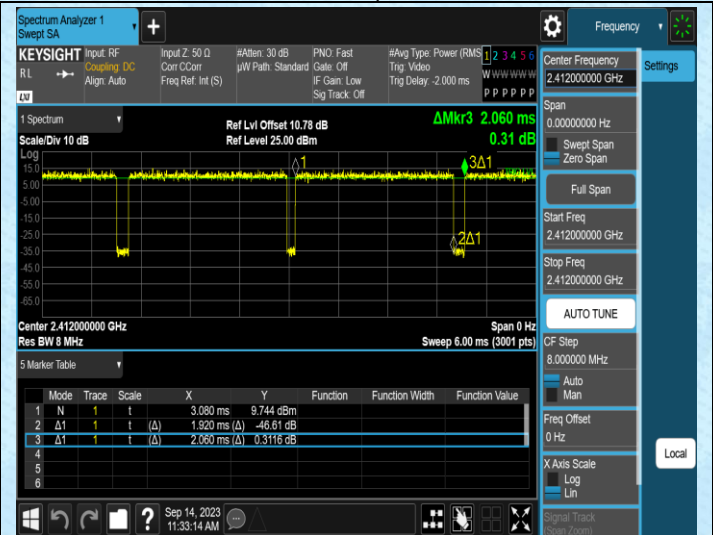
NTNV-11N20SISO-Ant2-2412
