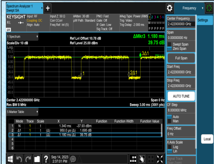
NTNV-11N40MIMO-Ant1-2422
