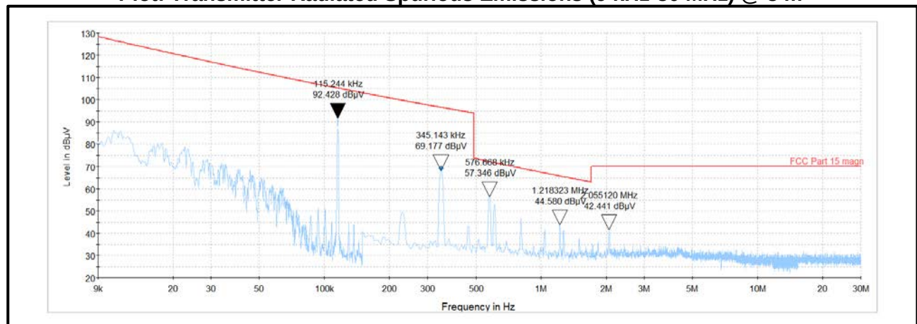
Plot: Transmitter Radiated Spurious Emissions (9 kHz-30 MHz) @ 3 m
