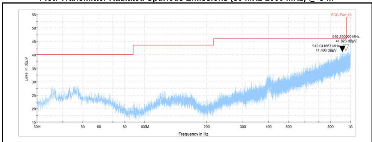
Plot: Transmitter Radiated Spurious Emissions (30 MHz-1000 MHz) @ 3 m
