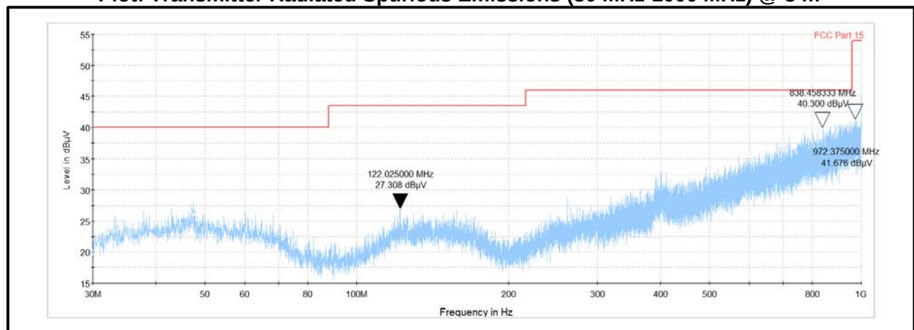
Plot: Transmitter Radiated Spurious Emissions (30 MHz-1000 MHz) @ 3 m
