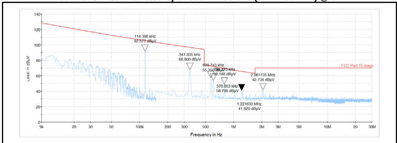
Plot: Transmitter Radiated Spurious Emissions (9 kHz-30 MHz) @ 3 m
