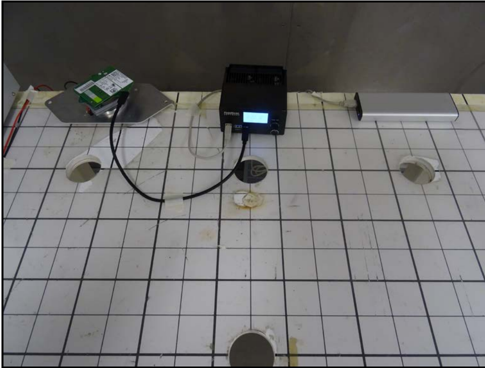
Photo 8 :AC Conducted Emissions Test Setup
