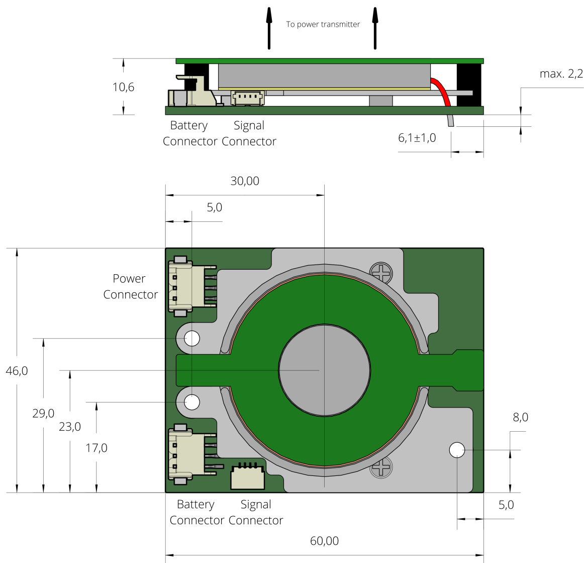
Figure 1: Dimensions
