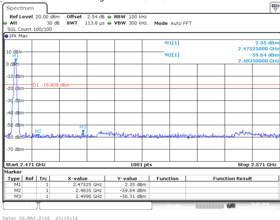
Band Edge NVNT 2.4G 2475MHz Ant1 Emission
