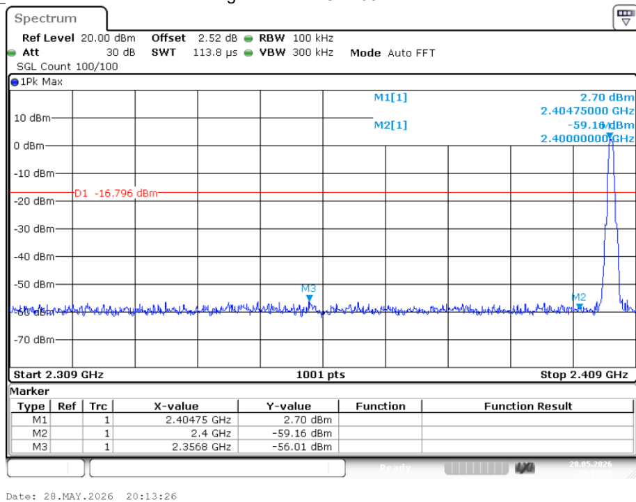
Band Edge NVNT 2.4G 2405MHz Ant1 Emission
