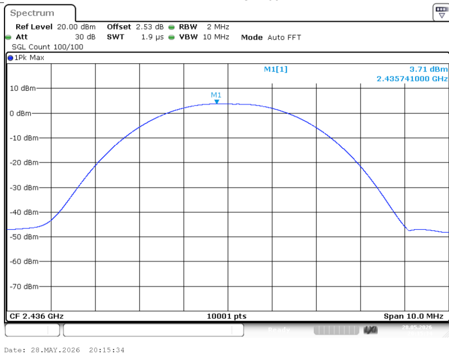
Peak Power NVNT 2.4G 2436MHz Ant1
