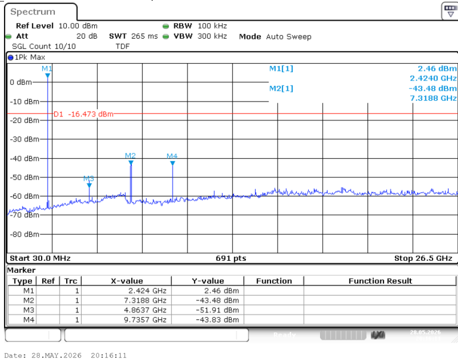
Tx. Spurious NVNT 2.4G 2436MHz Ant1 Emission
