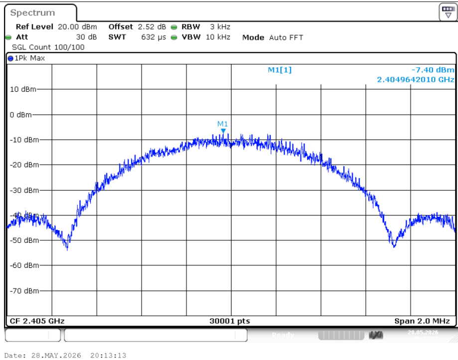
PSD NVNT 2.4G 2405MHz Ant1
