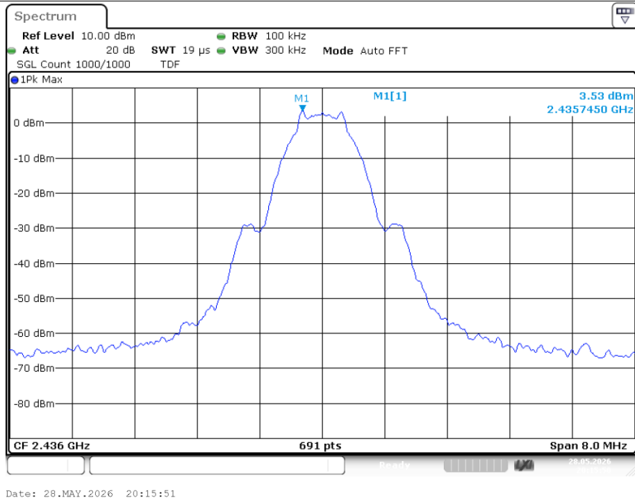
Tx. Spurious NVNT 2.4G 2436MHz Ant1 Ref
