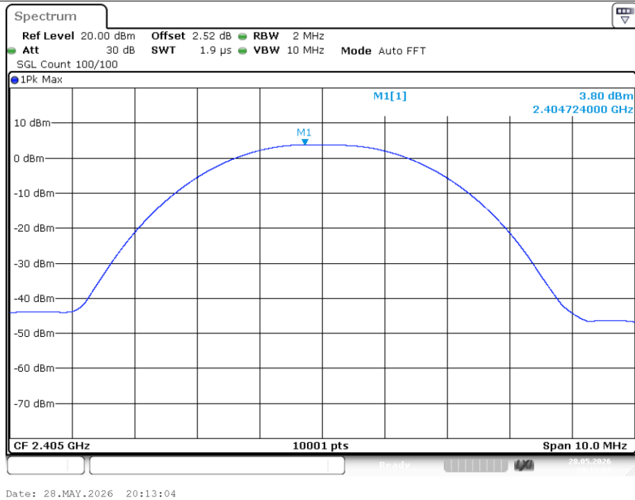
Peak Power NVNT 2.4G 2405MHz Ant1
