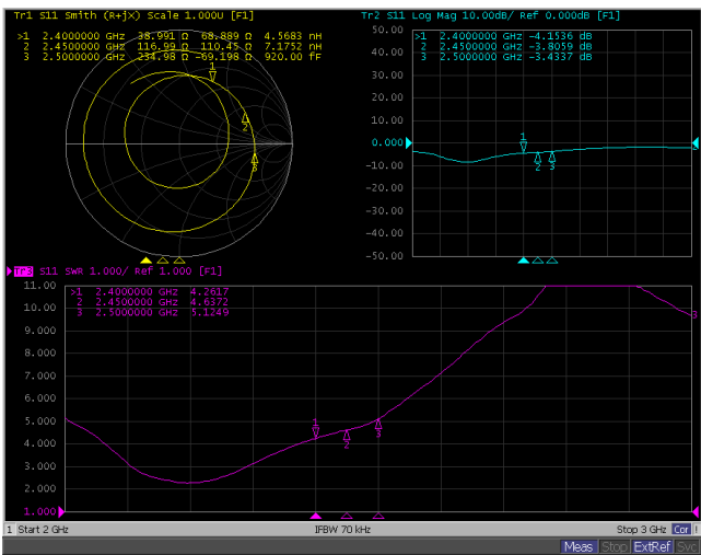
Original Antenna
