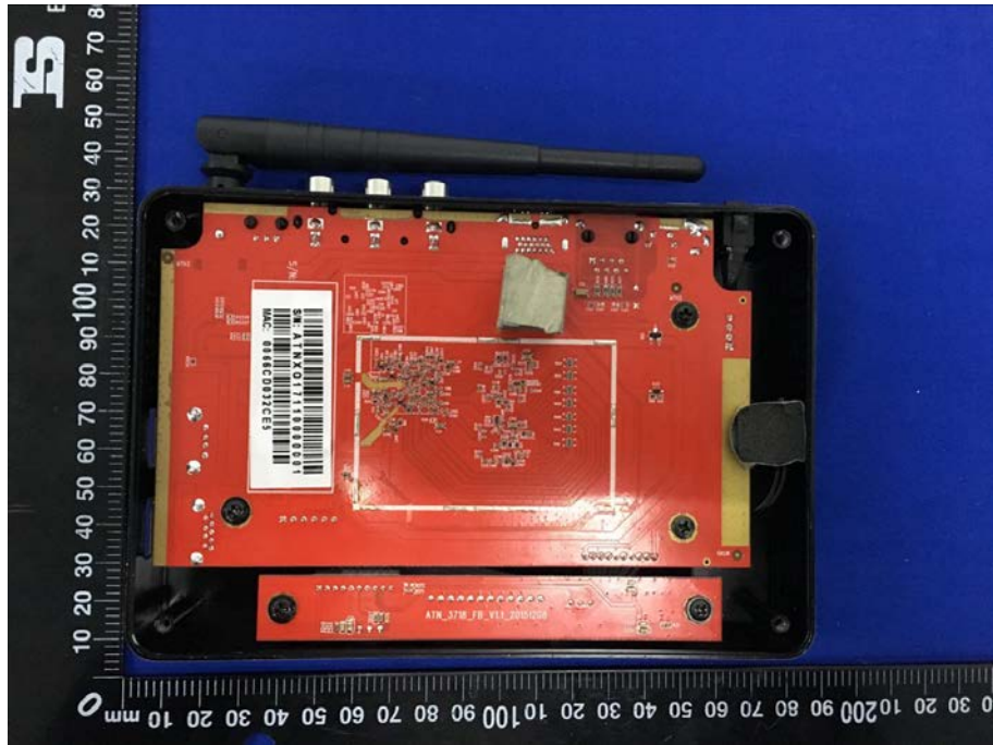
Internal Photos of EUT
