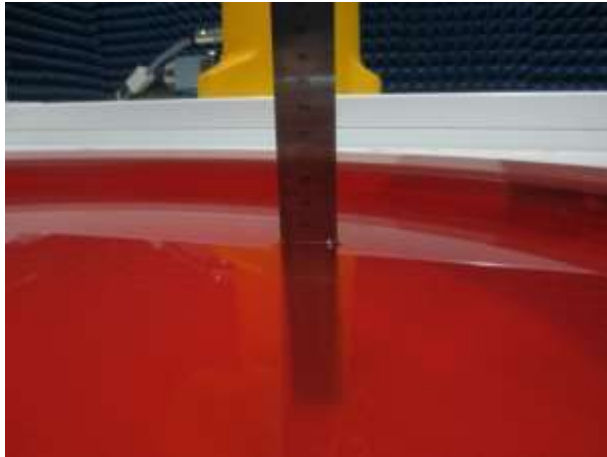
Fig. 9.2 Photo of Liquid Height for Head SAR of ELI V5.0 (700MHz~1000MHz) (depth>15cm)
