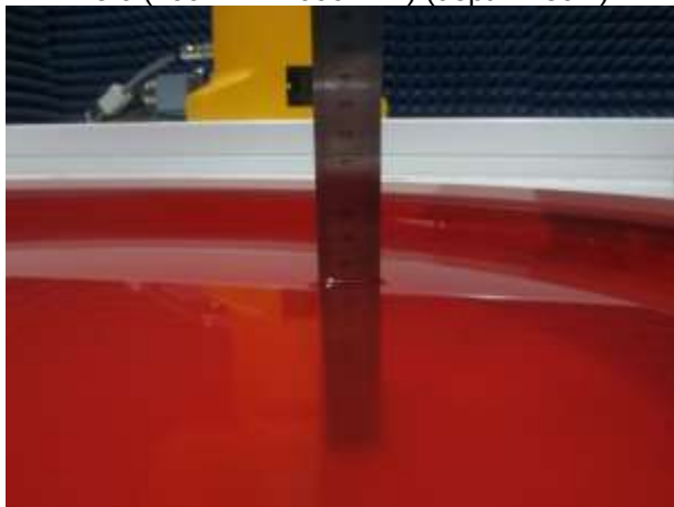
Fig. 9.4 Photo of Liquid Height for Head SAR of ELI V5.0 (1700MHz~1900MHz) (depth>15cm)
