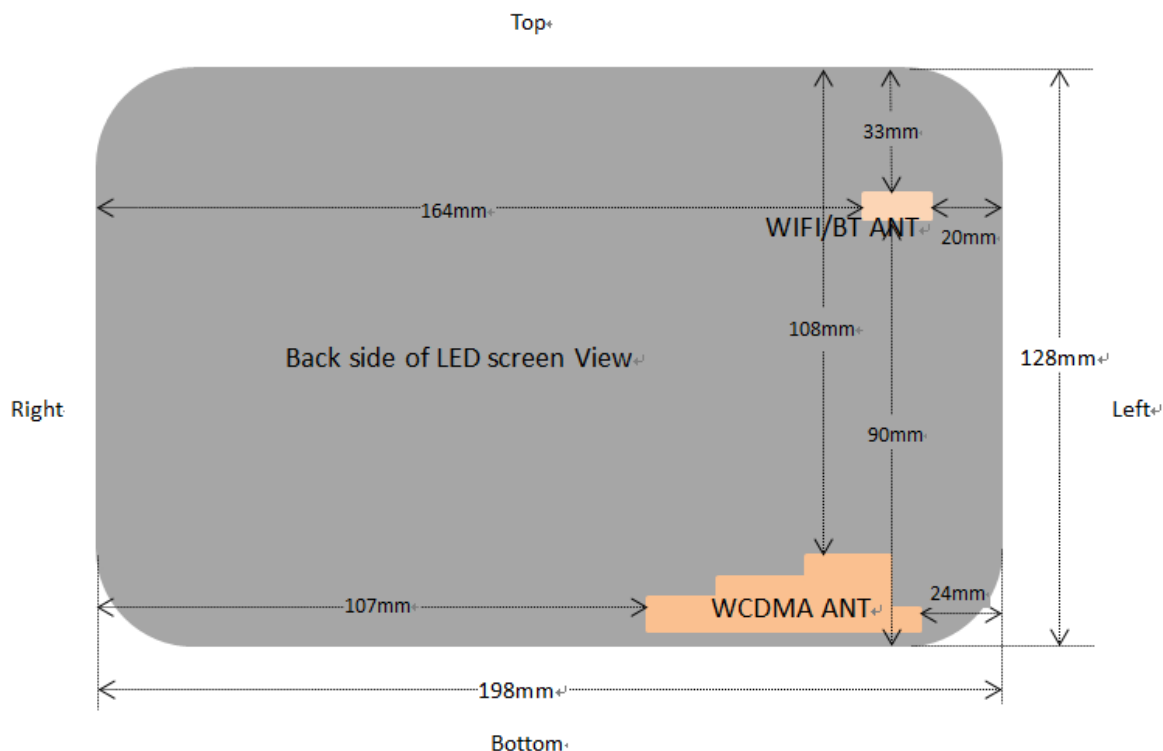
Fig.14.1 EUT Antenna Locations (Back side of LED screen View)
