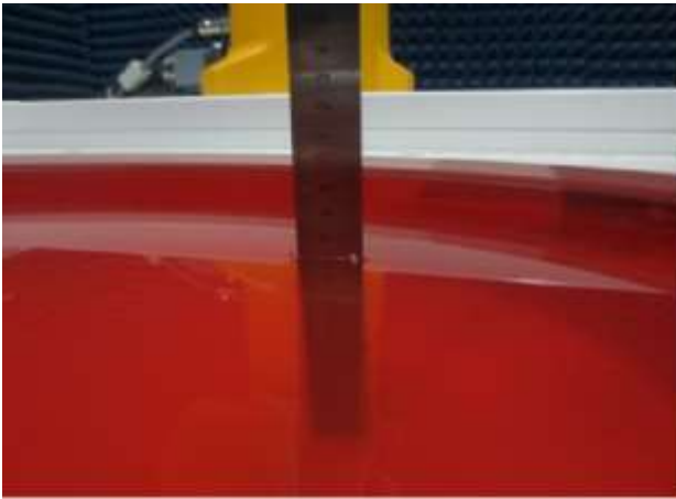
Fig. 9.6 Photo of Liquid Height for Head SAR of ELI V5.0 (2000MHz~2600MHz) (depth>15cm)
