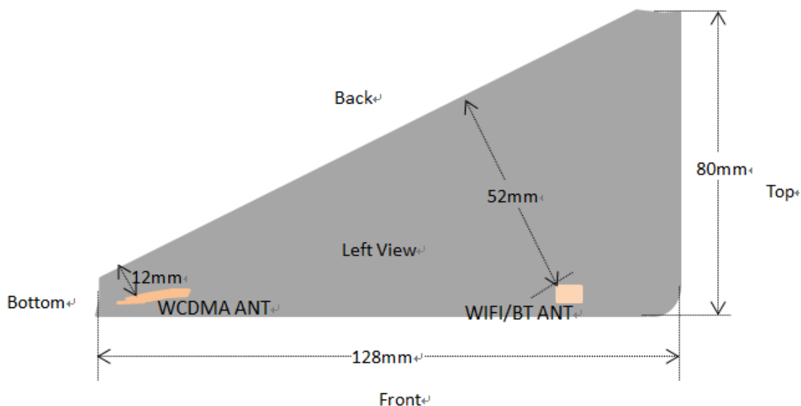
Fig.14.2 EUT Antenna Locations (Left View)
