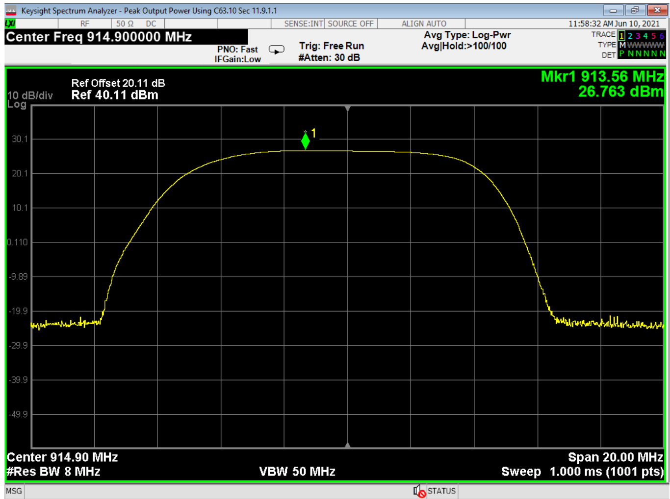
02 Output Power-Mid Channel
