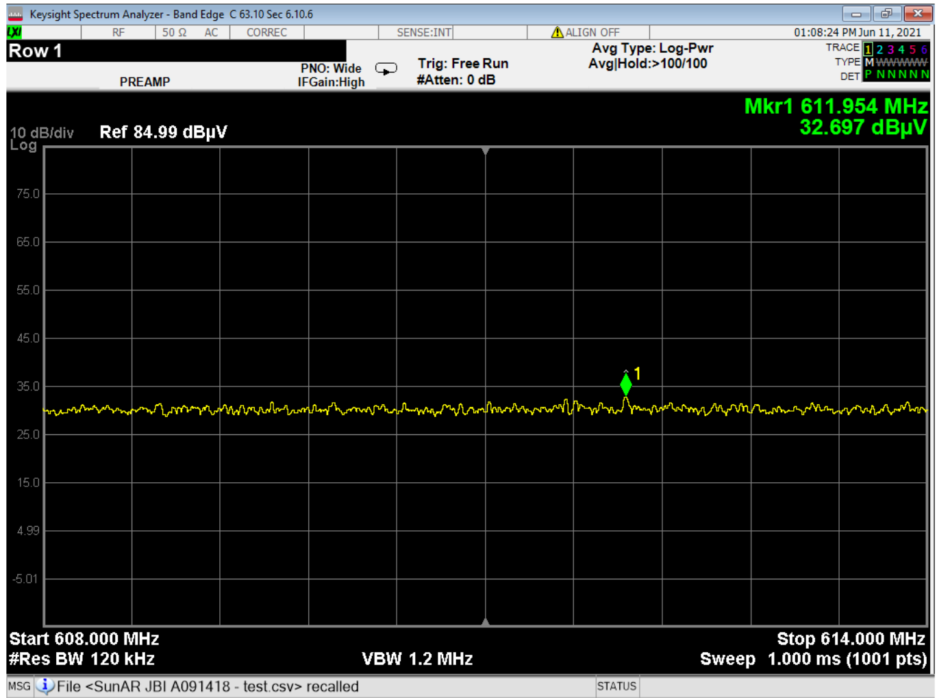
12 Radiated Restricted Bandedge-Low Channel
