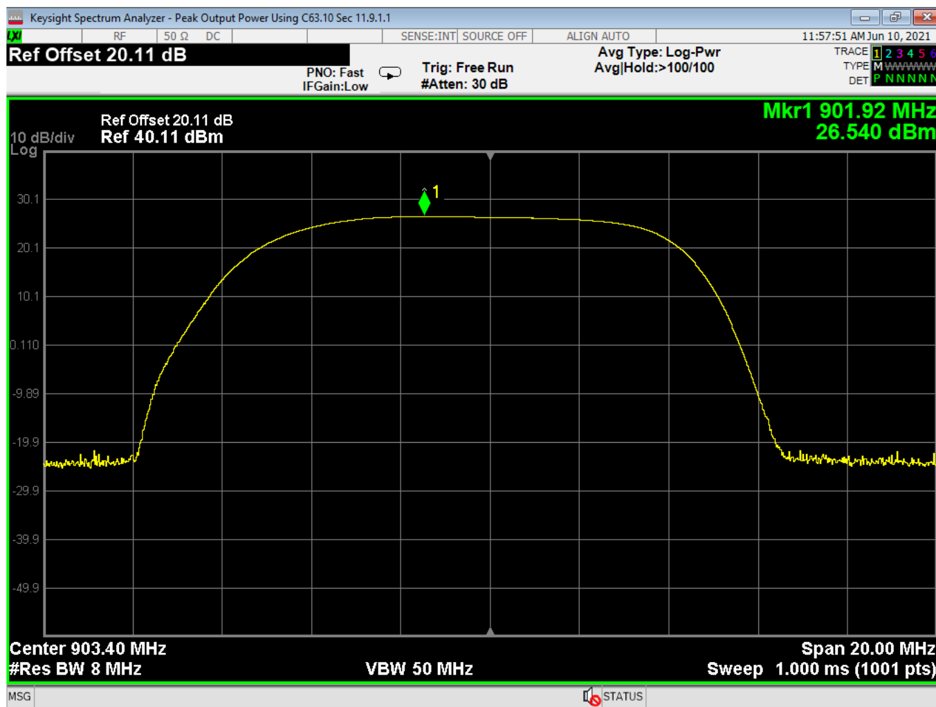
01 Output Power Low Channel
