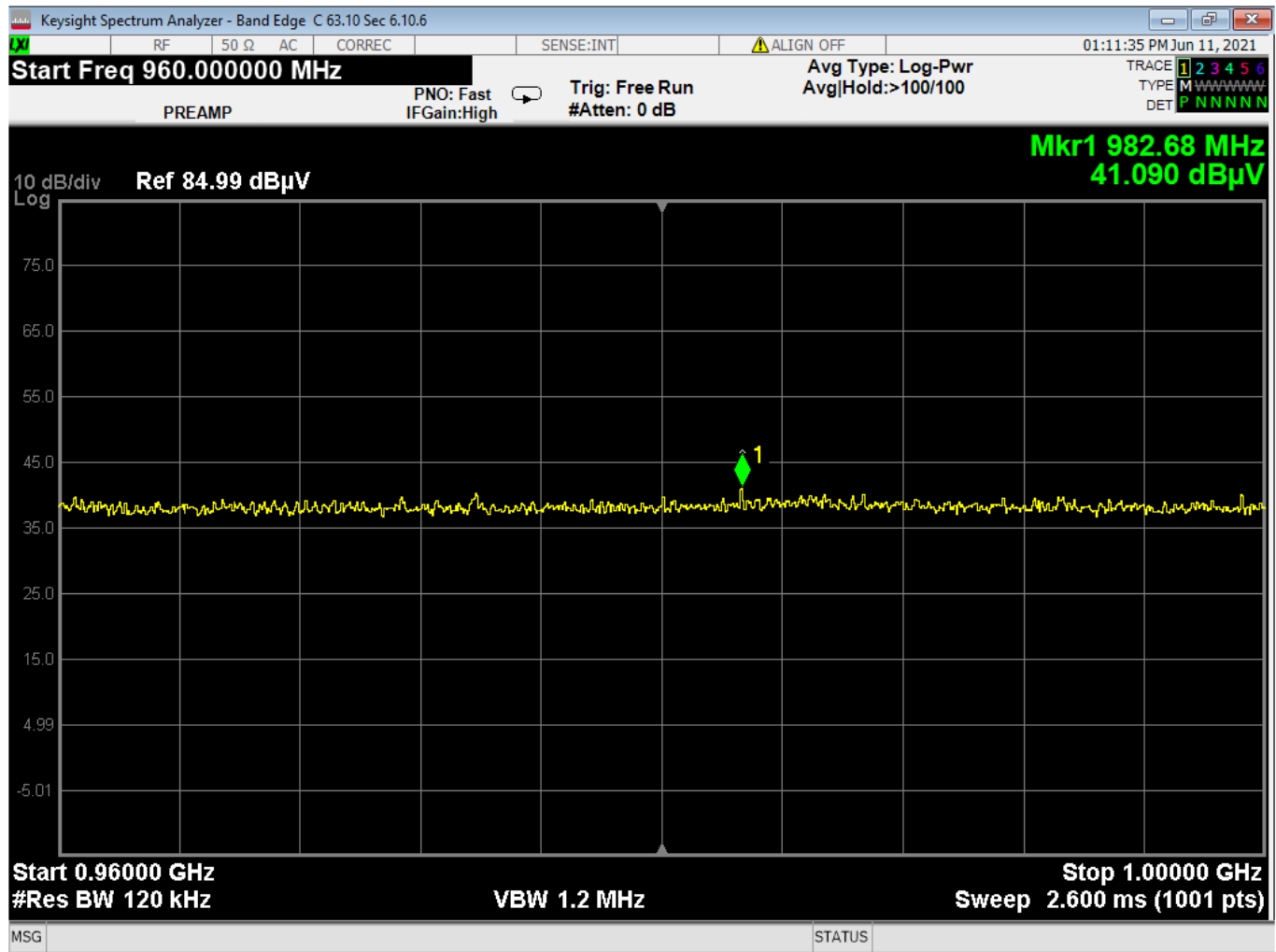
13 Radiated Restricted Bandedge-High Channel
