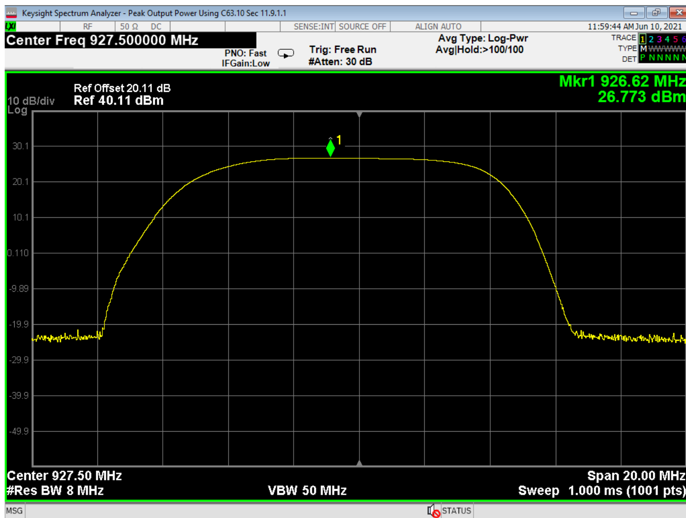
03 Output Power-High Channel
