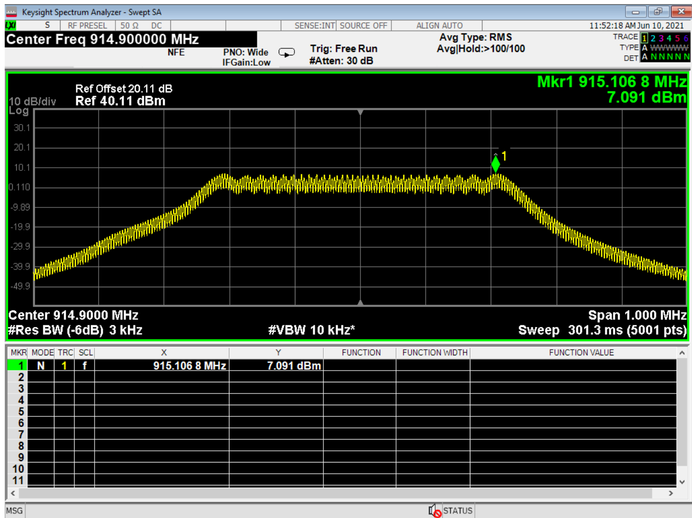
05 Power Spectral Density-Mid Channel, C63.10 Sec 11.10.3, AVGPSD-1
