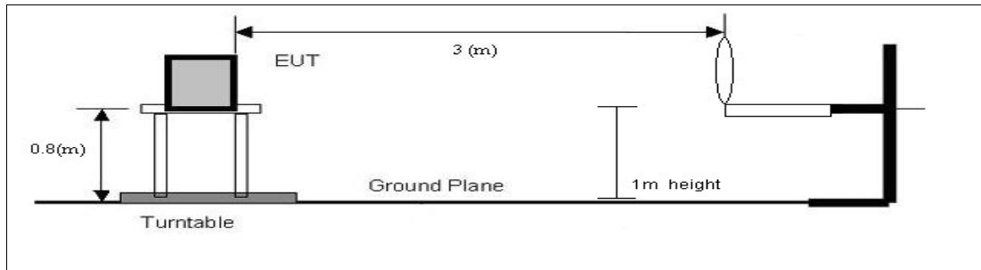
Figure 3.4 - Semi- Anechoic chamber diagram(0.009MHz - 30MHz)
