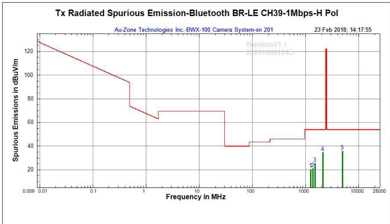
Figure 6.8 - Radiated Emission data(Ch 39, 1Mbps) -H-Pol
