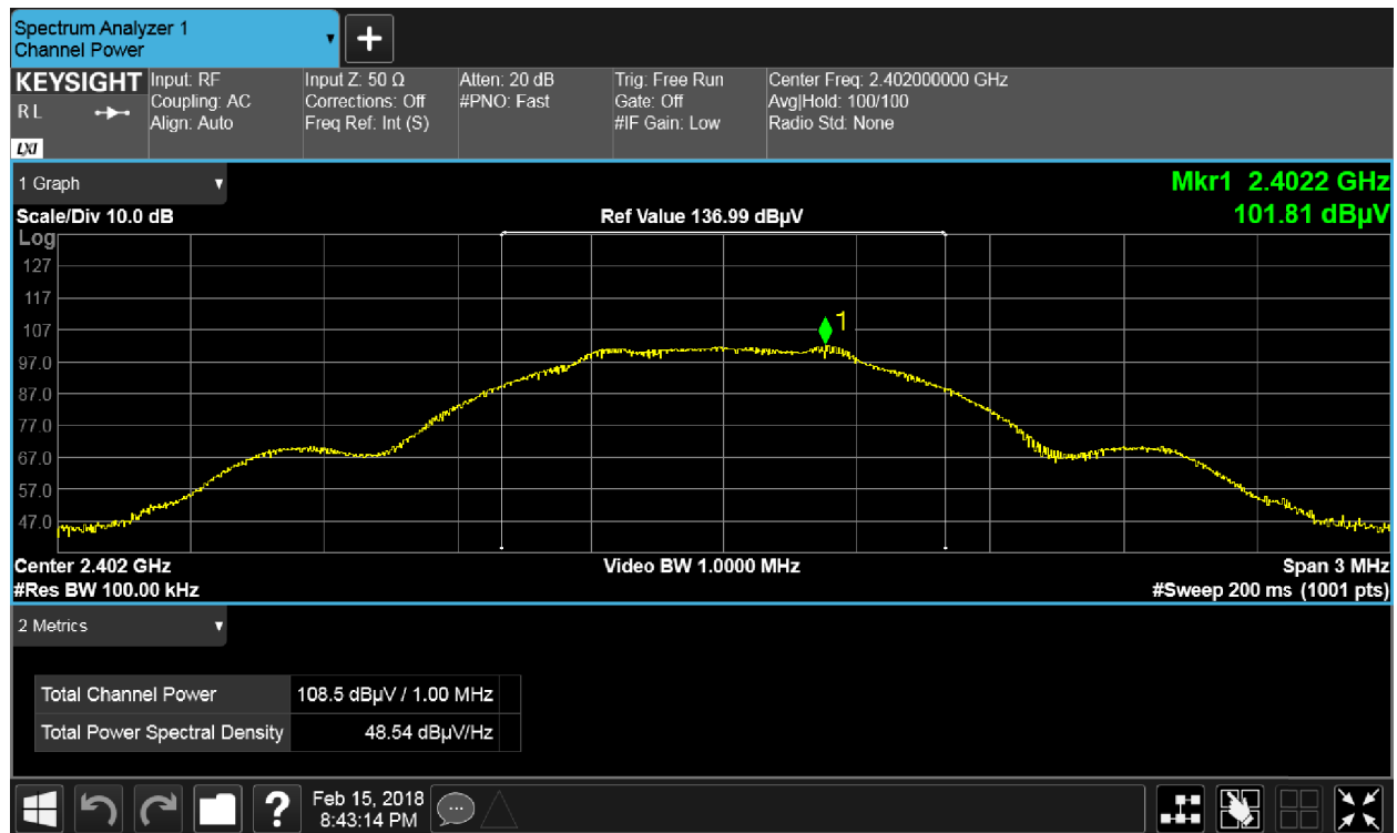
Figure 6.1 – Channel 0, Data rate 1M Data.
