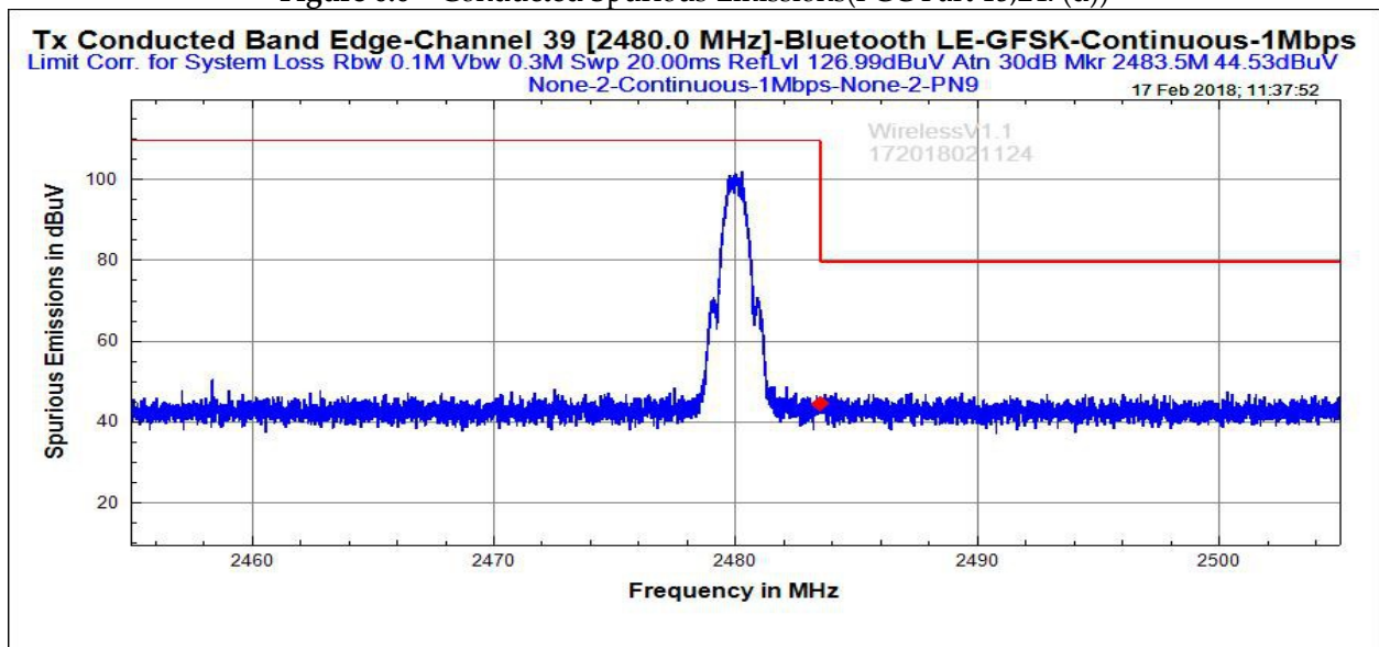
Figure 6.7 - Conducted Spurious Emissions(FCC Part 15,247(d))
