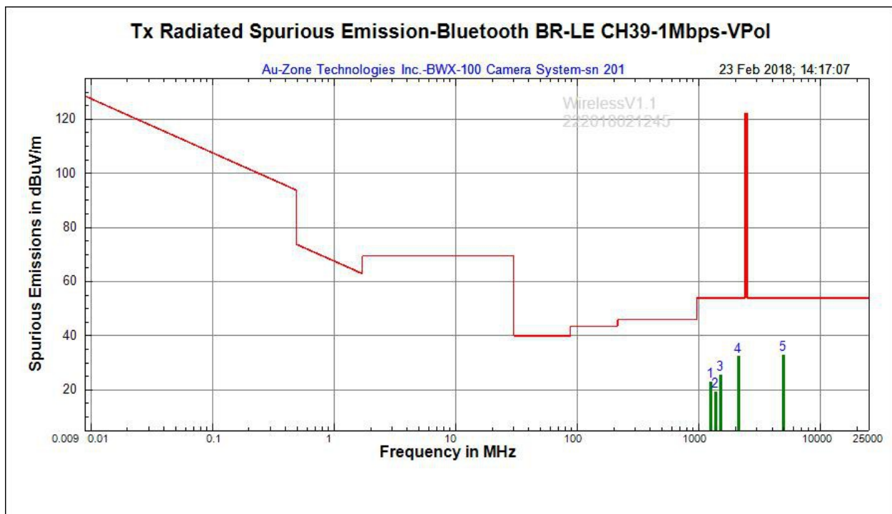
Figure 6.9 - Radiated Emission data(Ch 39, 1Mbps) – V-pol.
