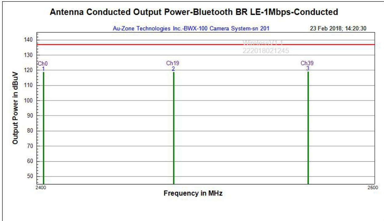
Figure 6.4 - Conducted Output Power (2400MHz - 2500MHz)
