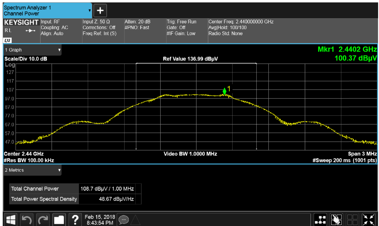
Figure 6.2 - Channel 19, Data rate 1M Data.
