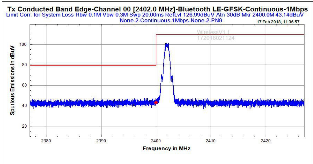
Figure 6.6 – Conducted Spurious Emissions(FCC Part 15,247(d))
