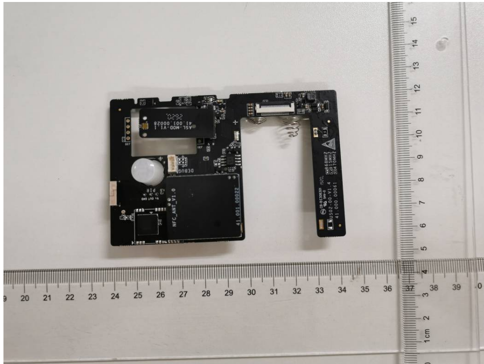
Model: AM100-915
