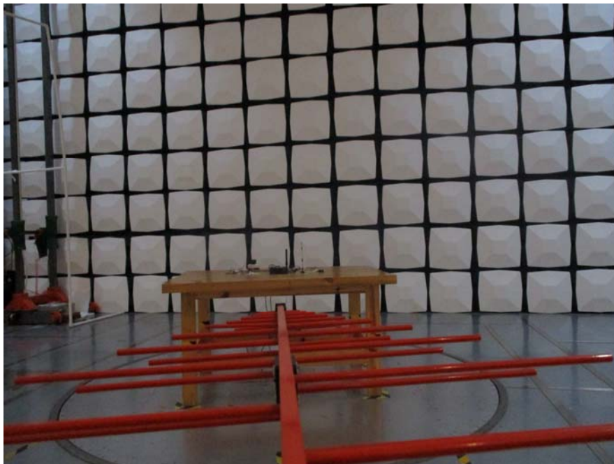
Radiated Emission Below 1GHz View For UR52
