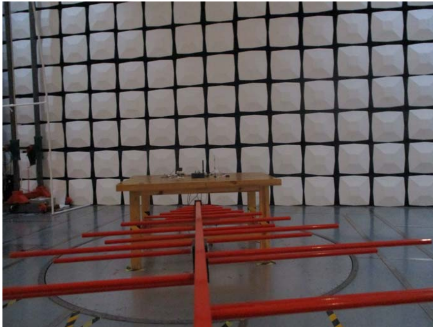
Radiated Emission Below 1GHz View For UR55
