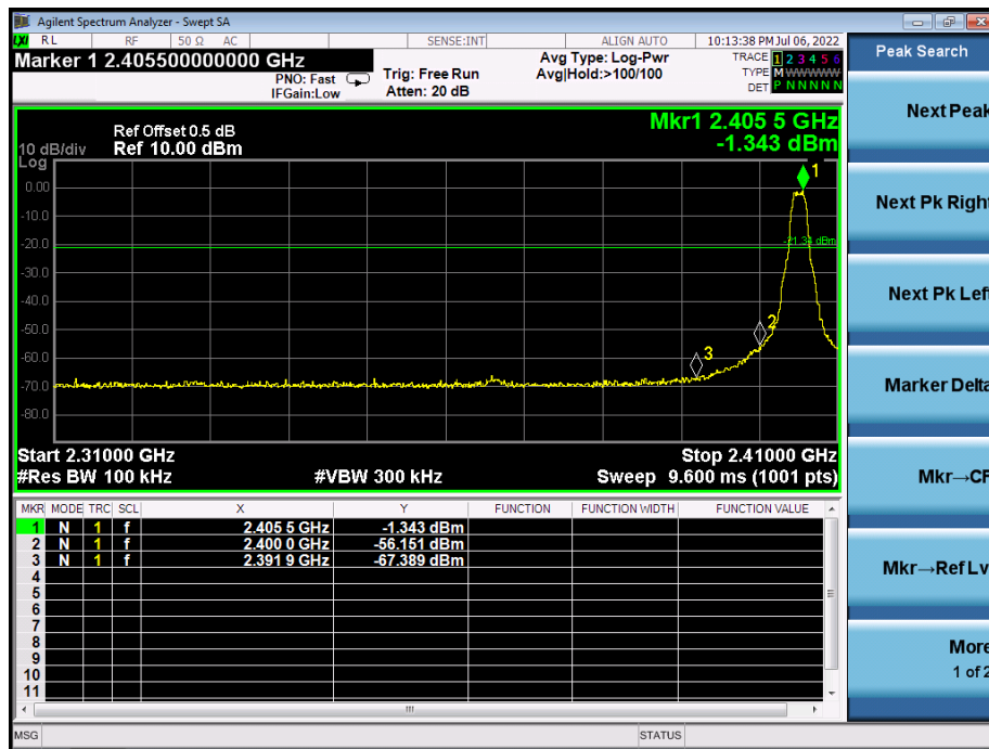
O-QPSK: Band Edge, Left Side
