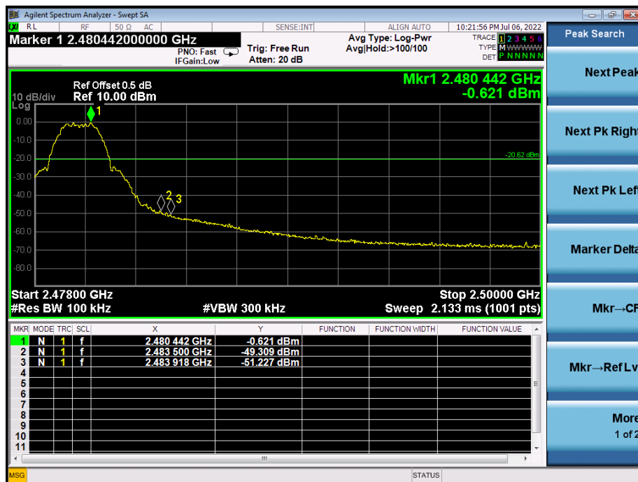
O-QPSK: Band Edge, Right Side
